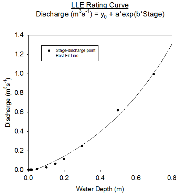
Figure A3.2: Stage-discharge relationship for the LLE hydrometric station. Values for y_0 , a , and b were determined to be -0.398, 0.3698 and 1.9111 respectively.
