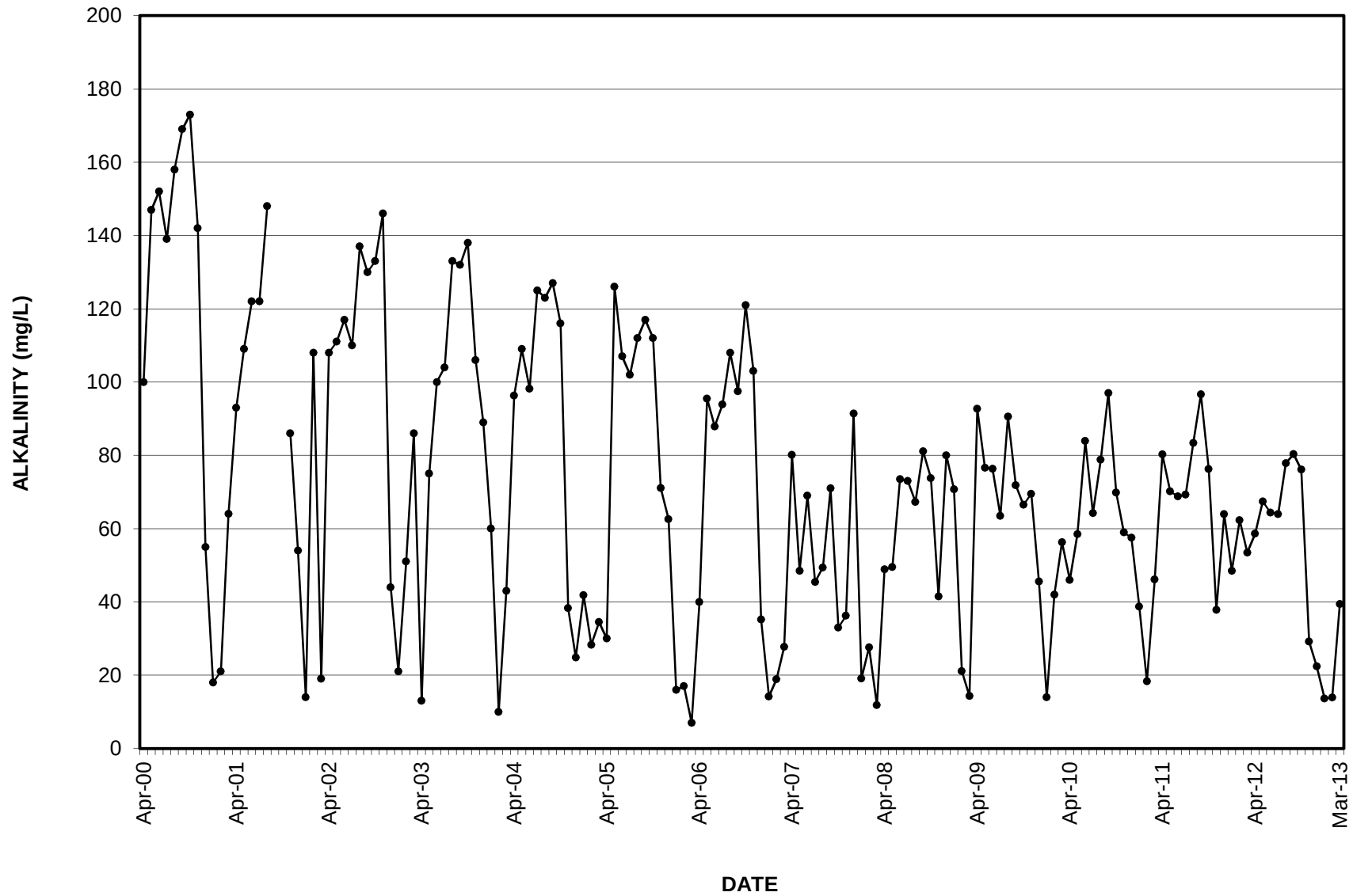
GRAPH 21 ALKALINITY SETTLING POND 1
