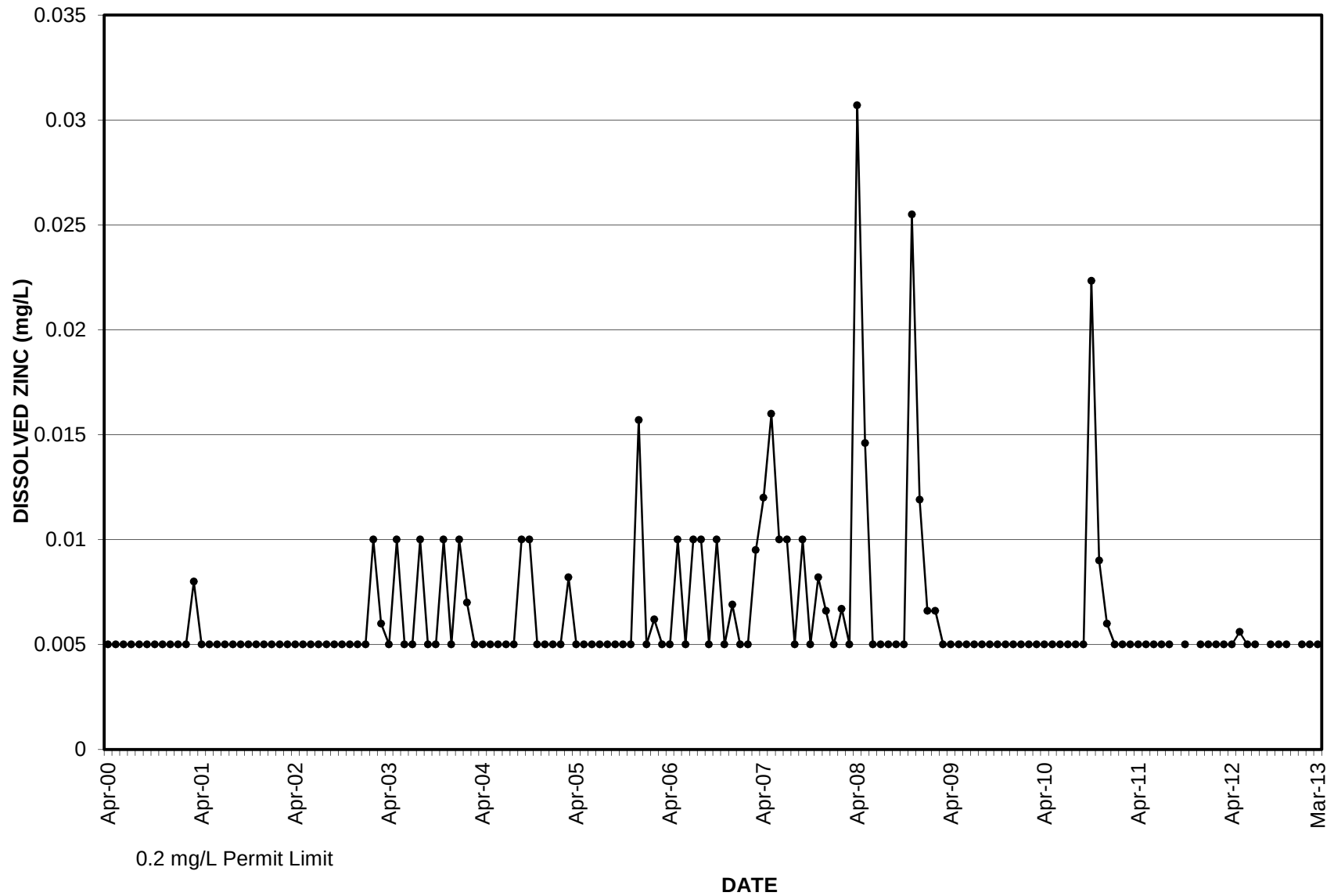
GRAPH 32 DISSOLVED ZINC SETTLING POND 1
