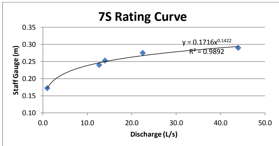
FIGURE 1: 7 SOUTH STAGE DISCHARGE RATING CURVE
