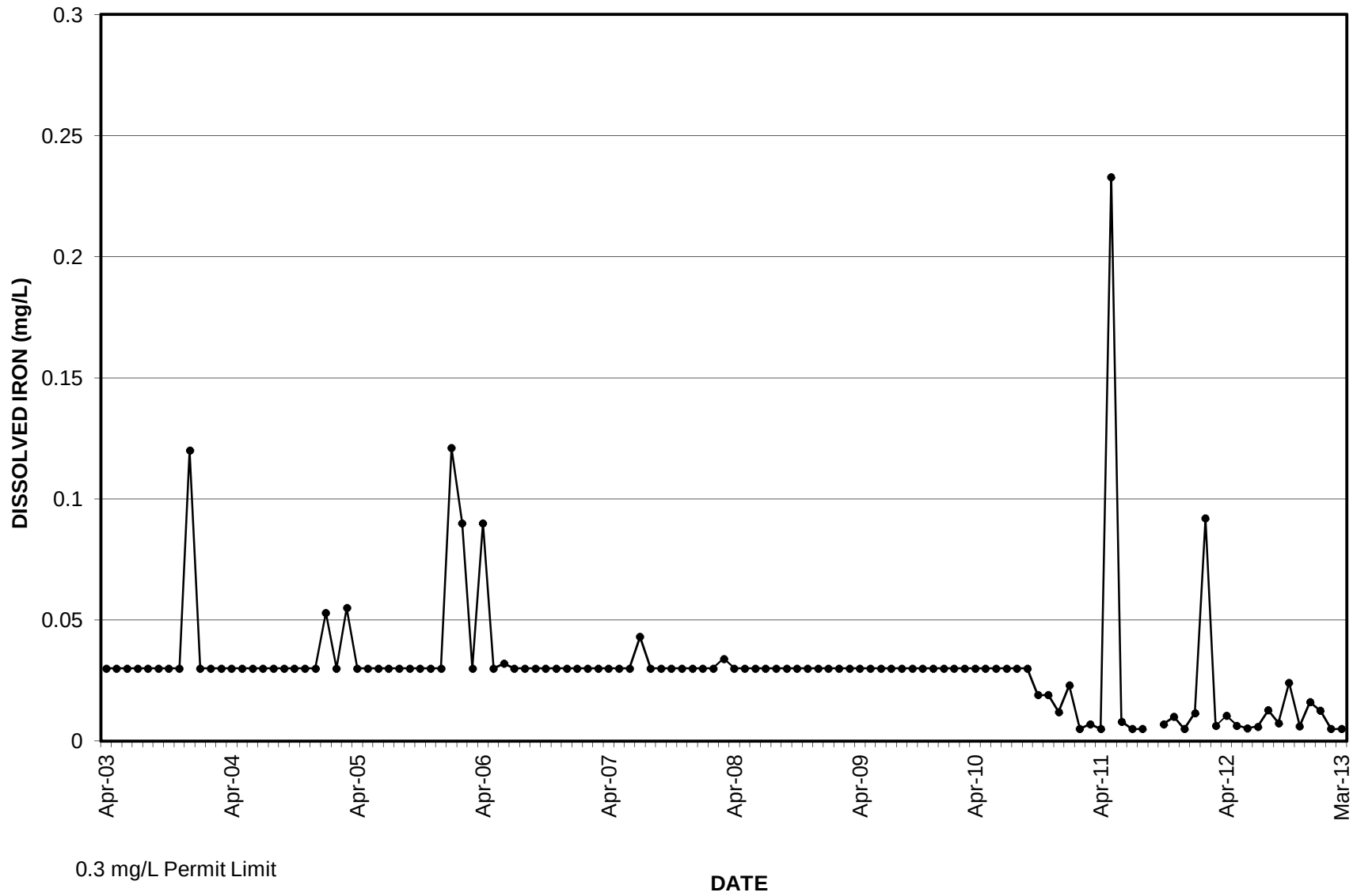
GRAPH 12 DISSOLVED IRON SETTLING POND 4
