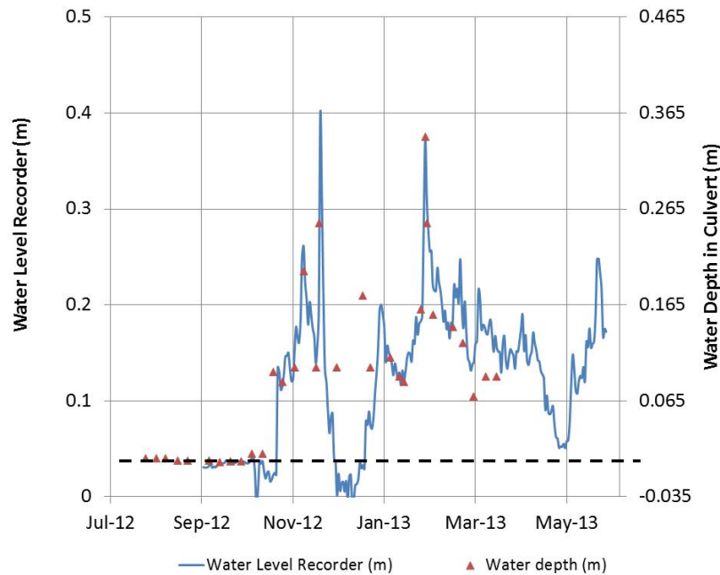
Figure A3.1: Relationship between continuous water level and spot measurements of water depth at LLE culvert for the period of record. The black dashed line indicates depth of zero discharge.
