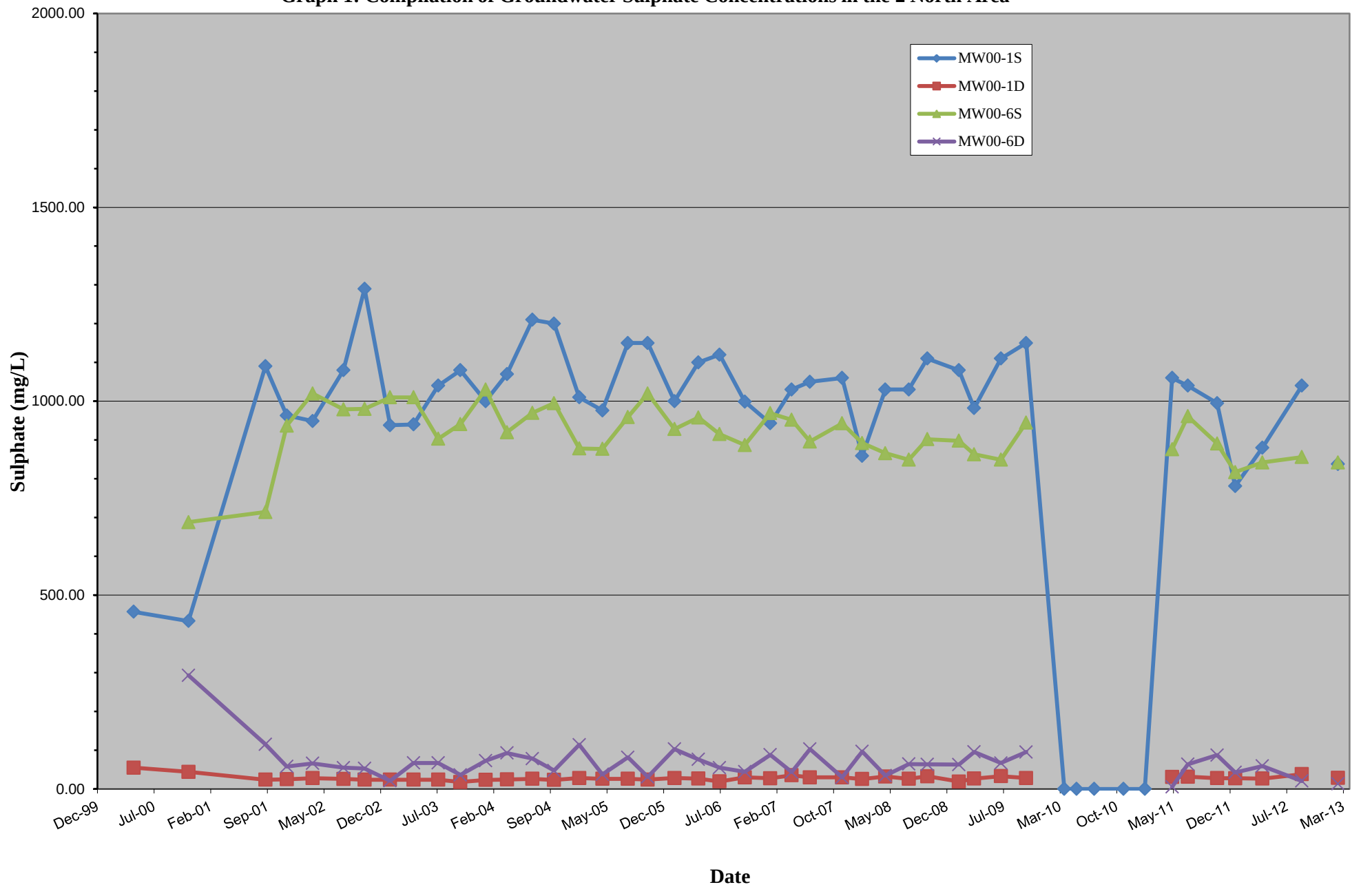
Graph 1: Compilation of Groundwater Sulphate Concentrations in the 2 North Area
