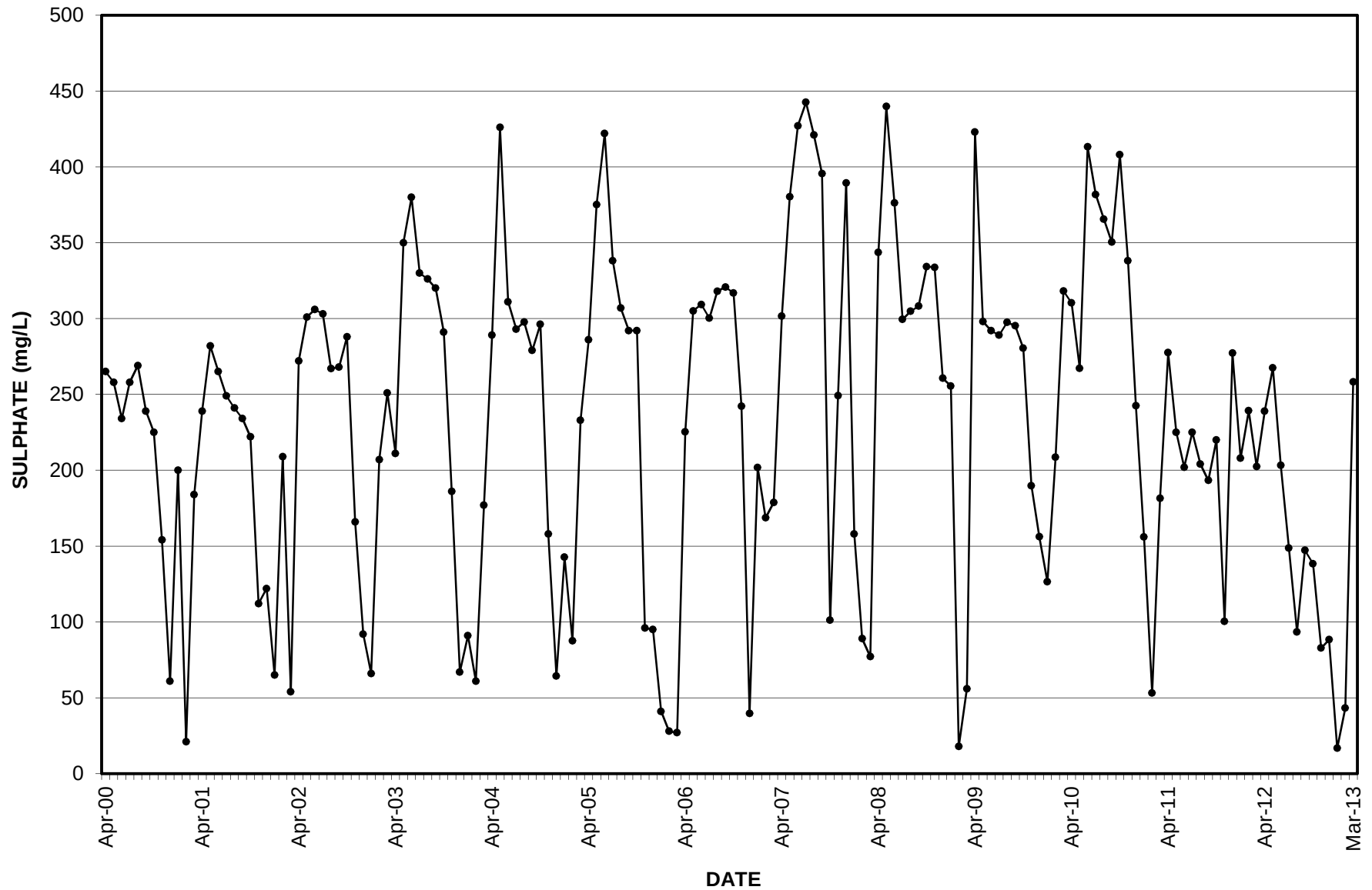
GRAPH 22 SULPHATE SETTLING POND 1
