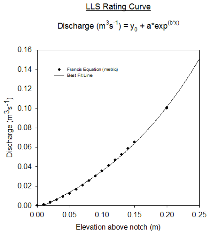
Figure A2.2: Stage-discharge relationship for the LLS hydrometric station. Values for y_0 , a , and b were determined to be -0.0547, 0.0520 and 5.5017 respectively.
