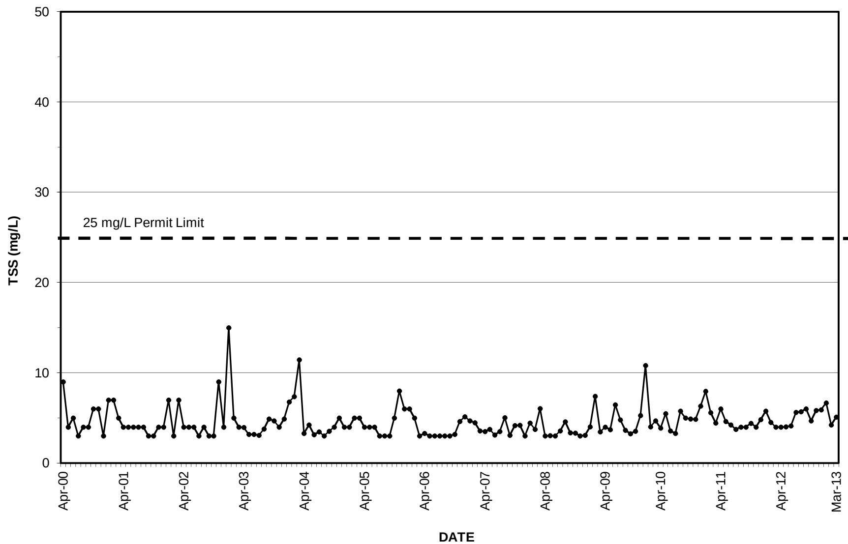
GRAPH 3 TOTAL SUSPENDED SOLIDS SETTLING POND 4
