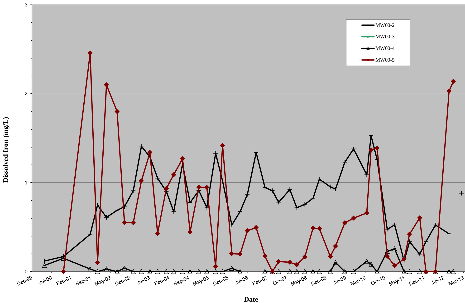
Graph 7: Compilation of Groundwater Dissolved Iron Concentrations in the 3 South Pit Area
