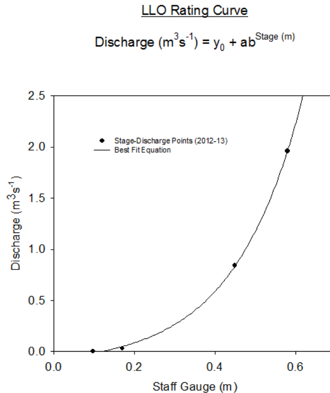
FigureA1.2: Stage-discharge relationship for the LLO hydrometric station. Values for y_0 , a , and b were determined to be -0.1381, 0.0687 and 363.1808 respectively.
