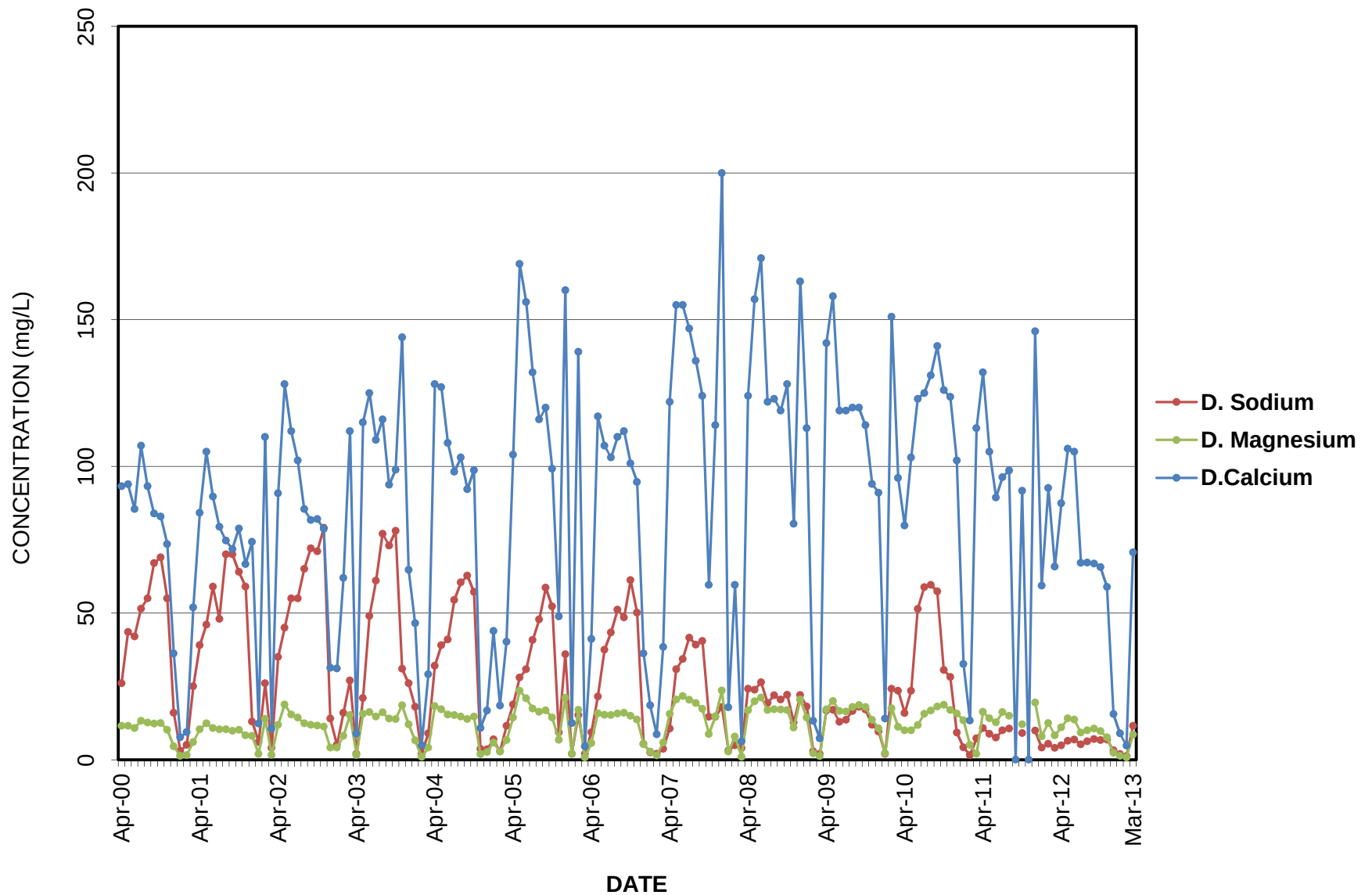
GRAPH 33 DISSOLVED CALCIUM/MAGNESIUM/SODIUM SETTLING POND 1
