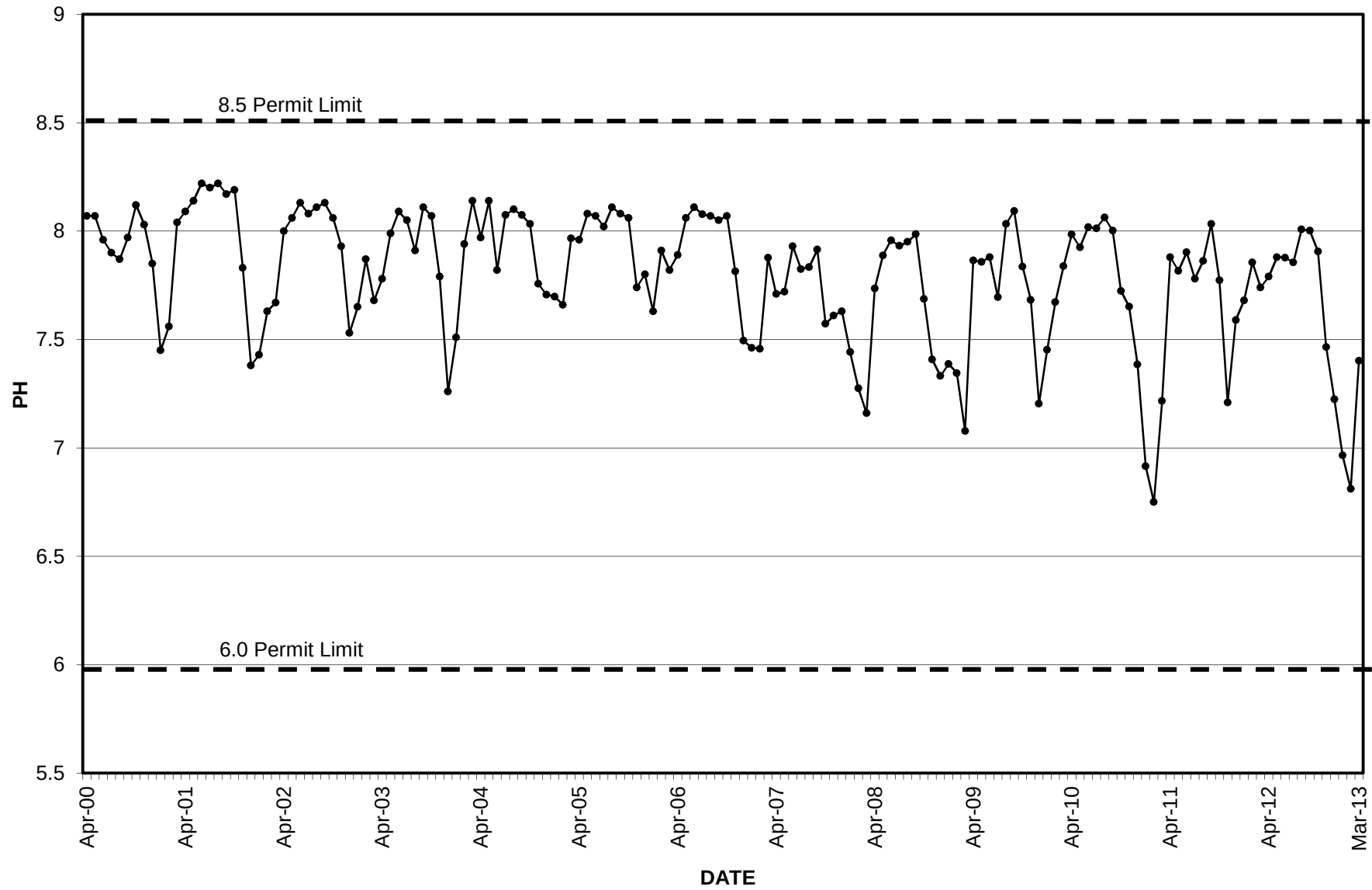
GRAPH 19 PH SETTLING POND 1
