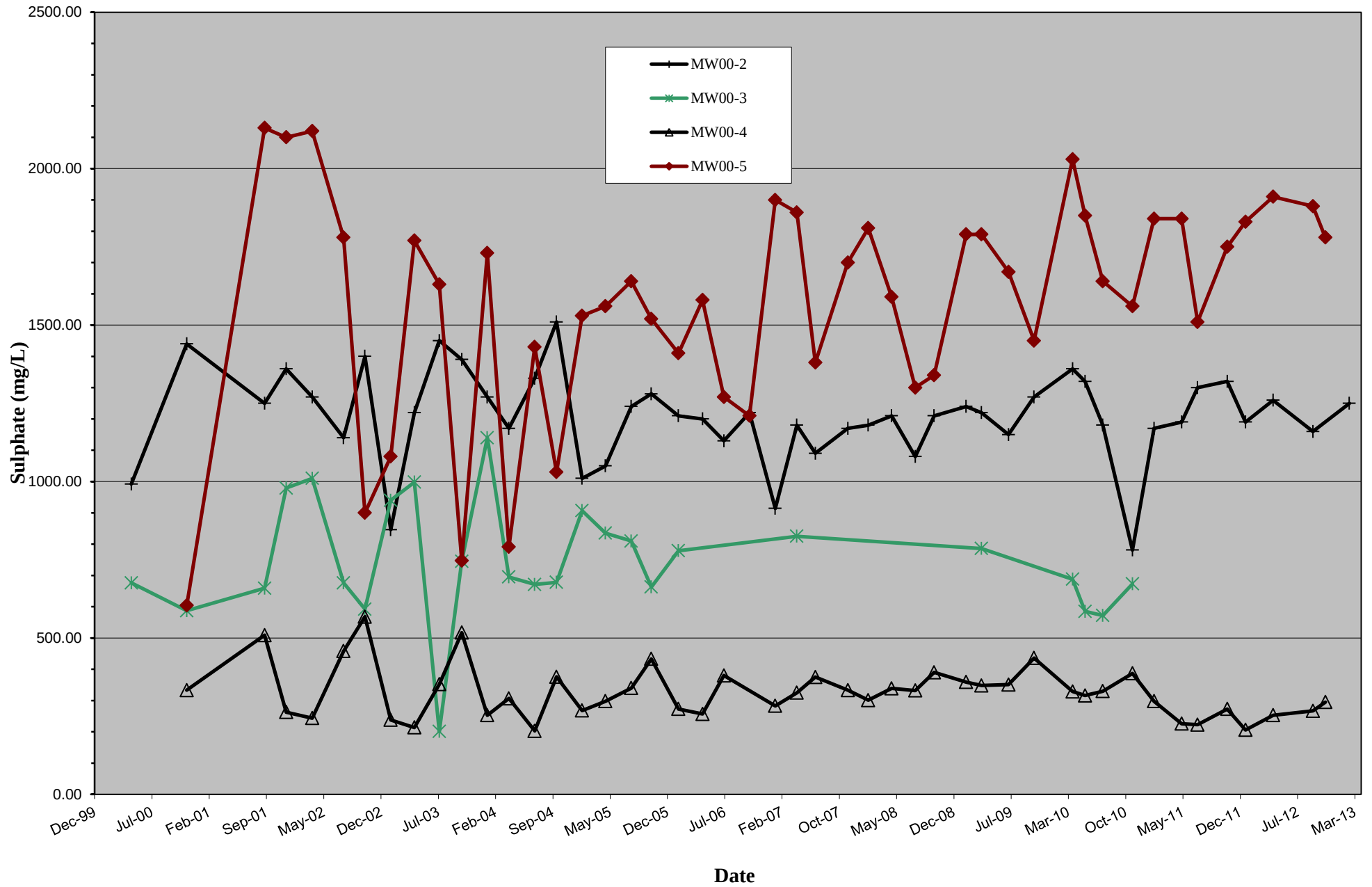
Graph 4: Compilation of Groundwater Sulphate Concentrations in the 3 South Pit Area
