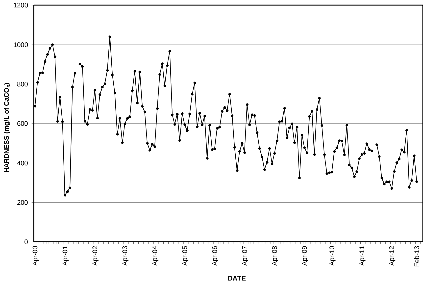
GRAPH 1 HARDNESS SETTLING POND 4
