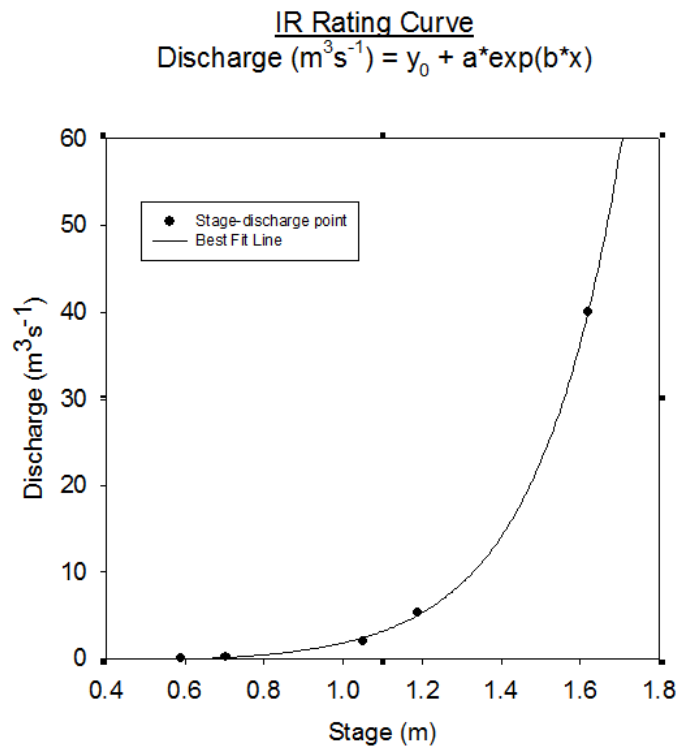
Figure A6.2: Stage-discharge relationship for the IR hydrometric station. Values for y_0 , a , and b were determined to be -0.4084, 0.0214 and 4.6573 respectively.
