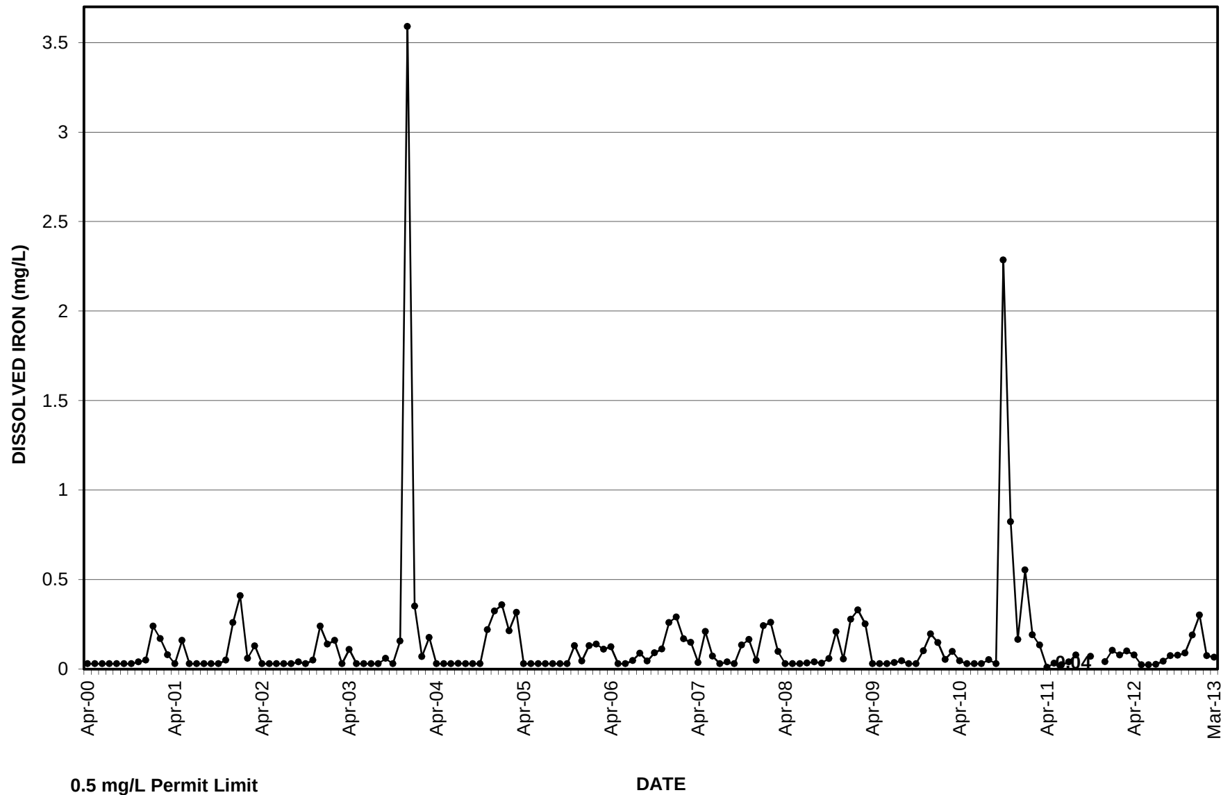
GRAPH 29 DISSOLVED IRON SETTLING POND 1
