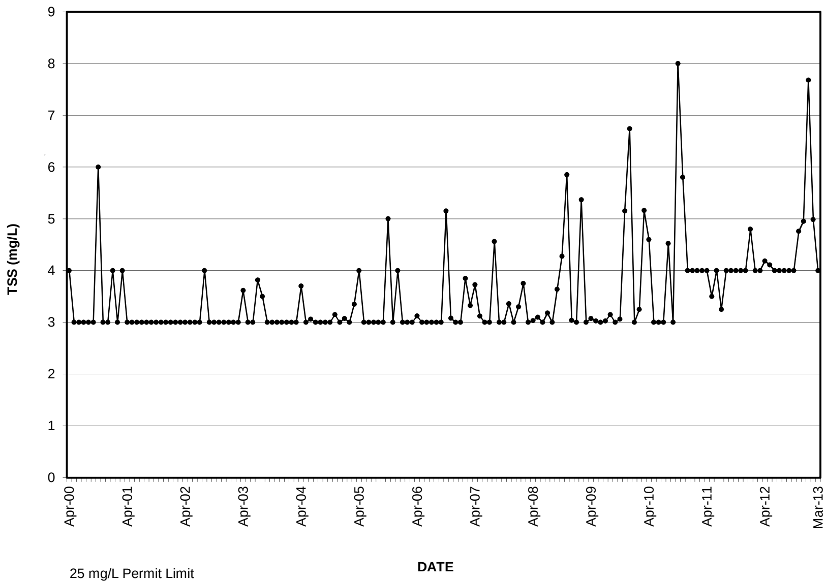
GRAPH 20 TOTAL SUSPENDED SOLIDS SETTLING POND 1
