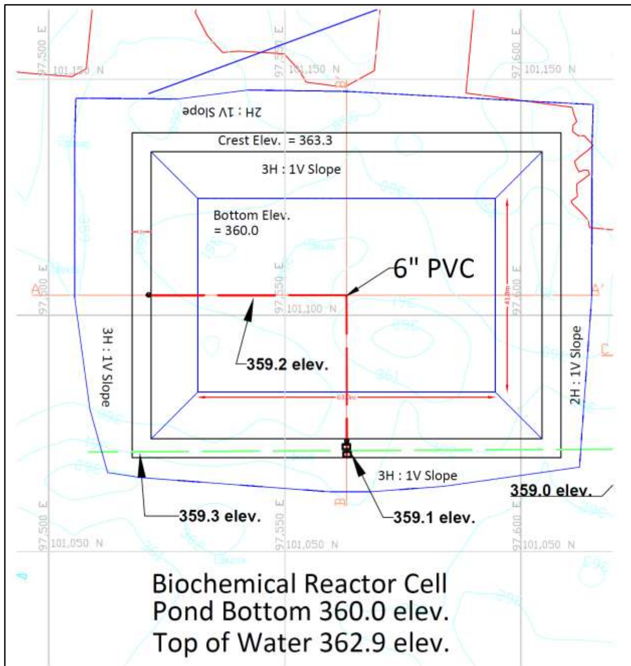
Figure 1: BCR Cell Construction Design – Layout
