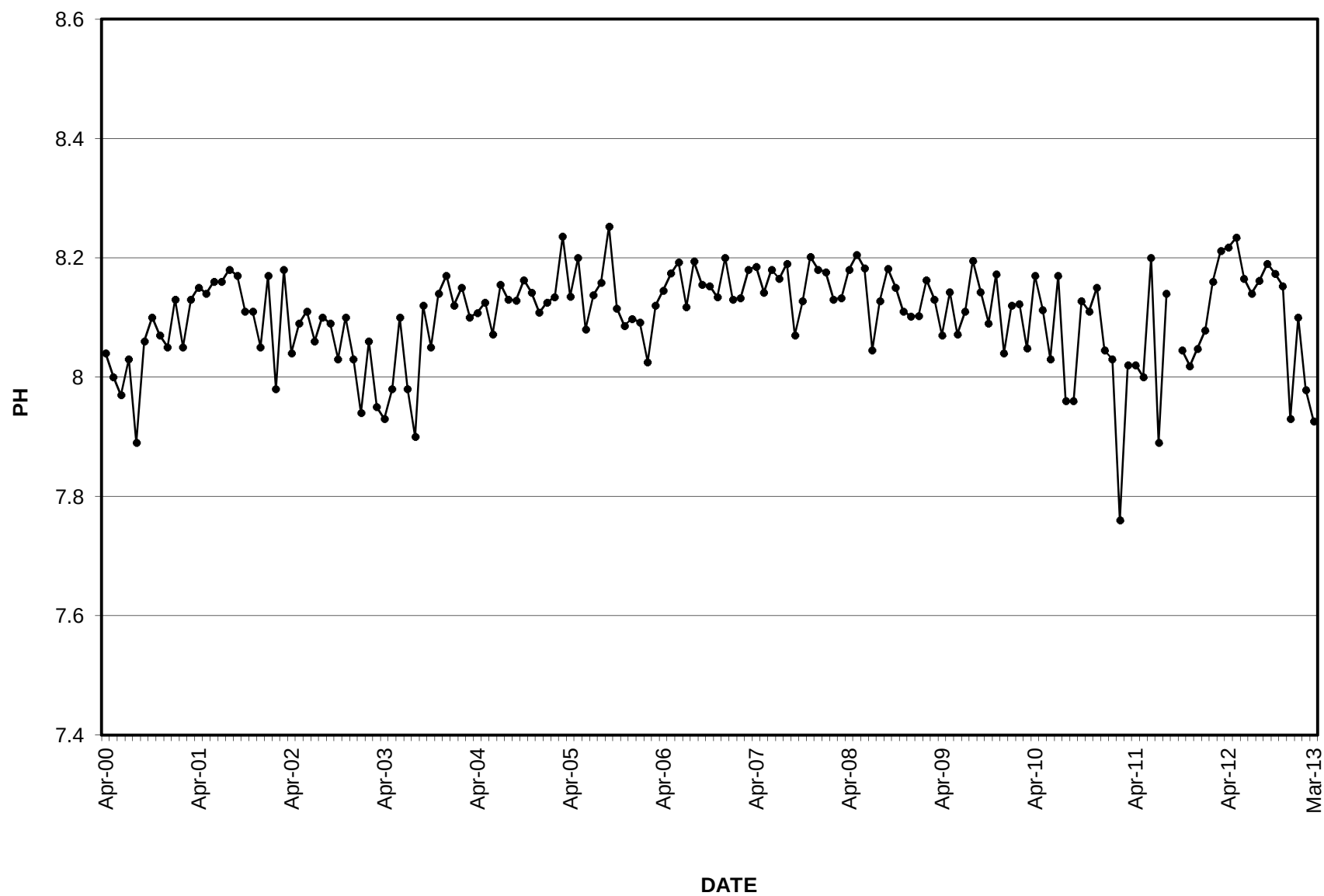
GRAPH 35 PH NORTH PIT SUMP (WP)
