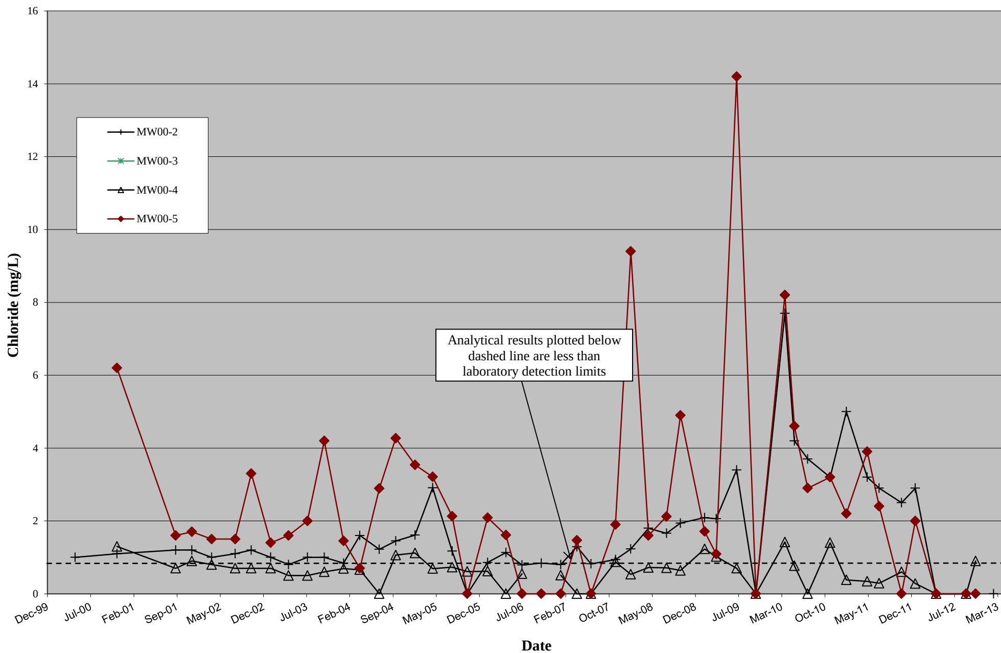
Graph 6: Compilation of Groundwater Chloride Concentrations in the 3 South Area
