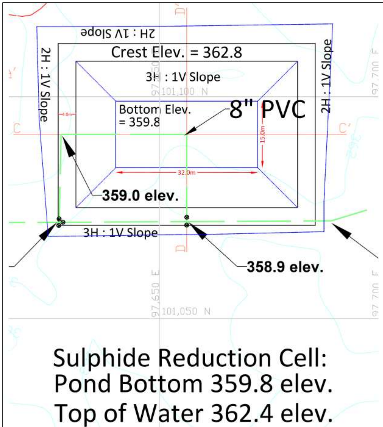
Figure 2: Sulphide Polish Cell Construction Design – Layout
