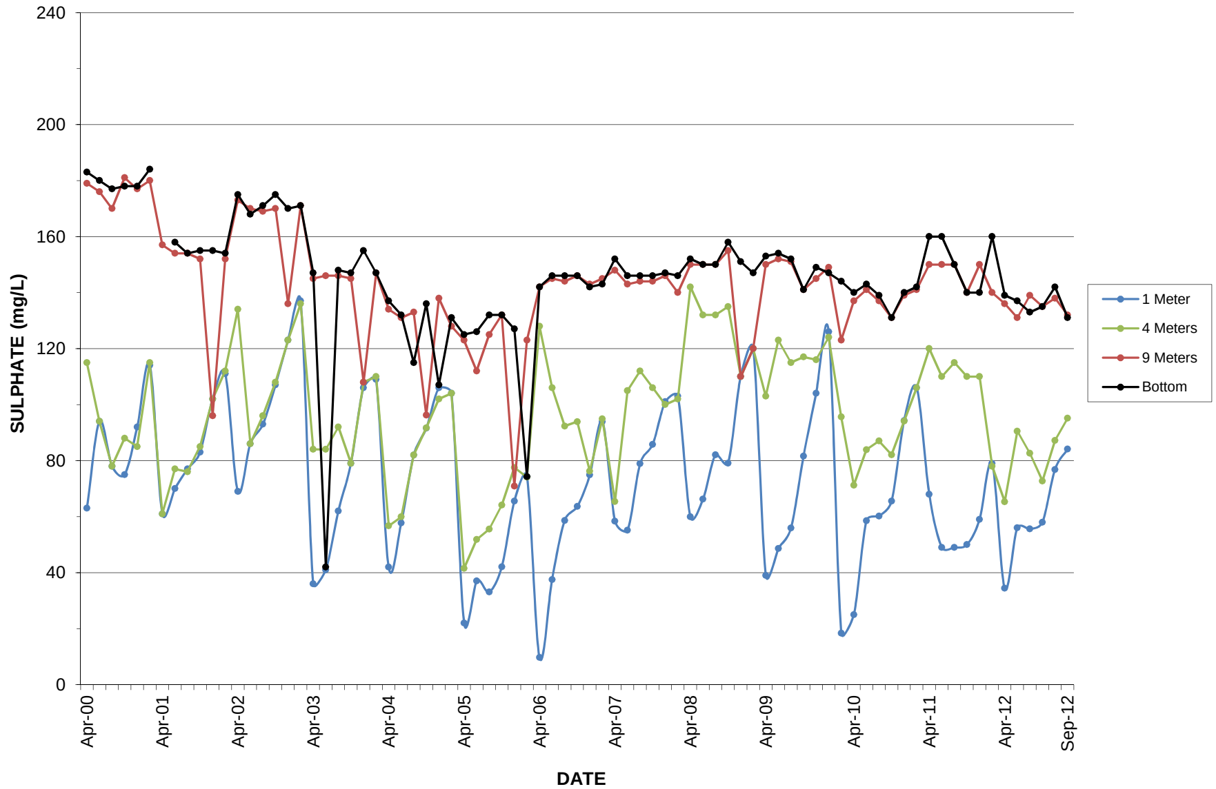
GRAPH 49 LONG LAKE SULPHATE
