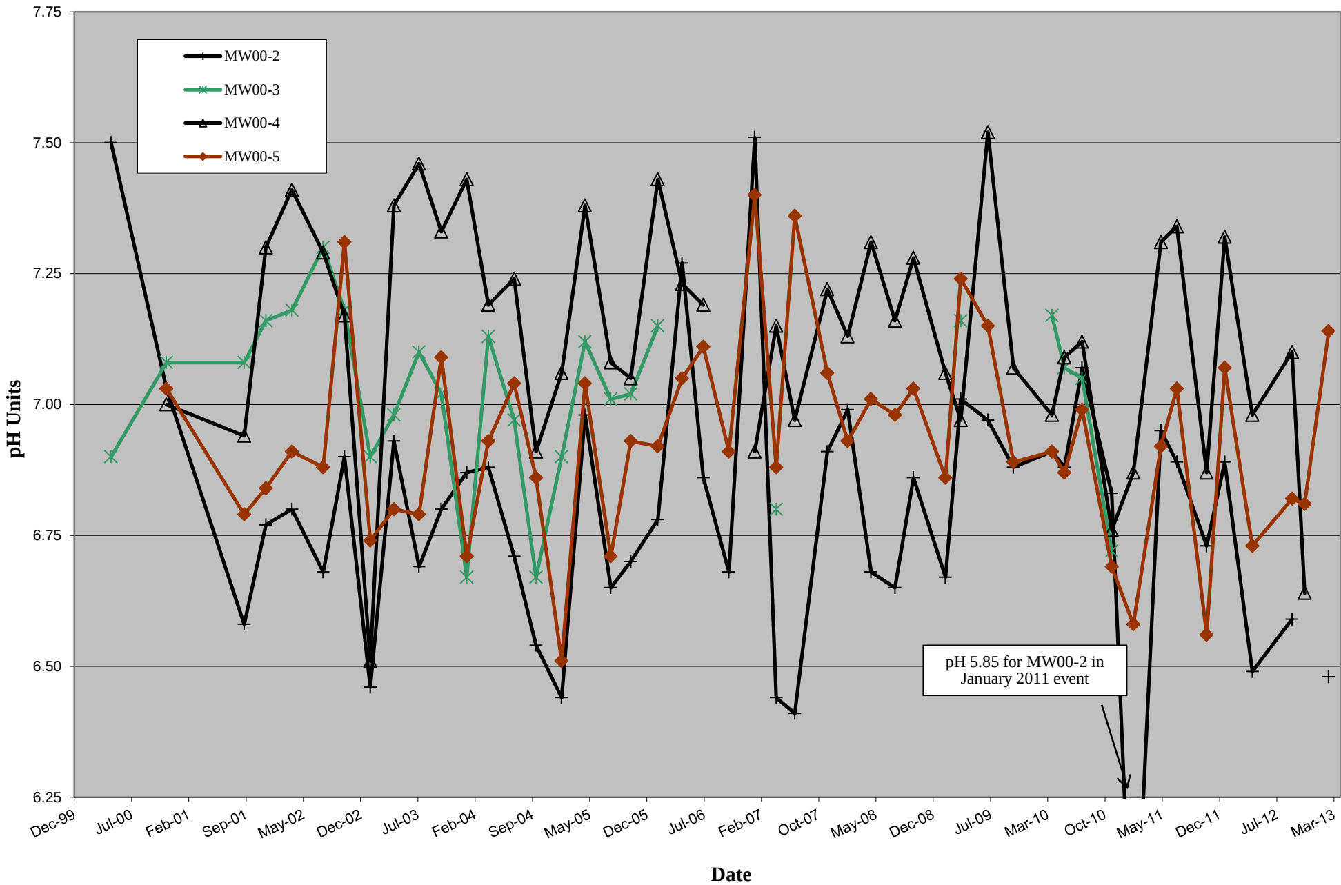
Graph 5: Compilation of Field Measured pH in Groundwater in the 3 South Area
