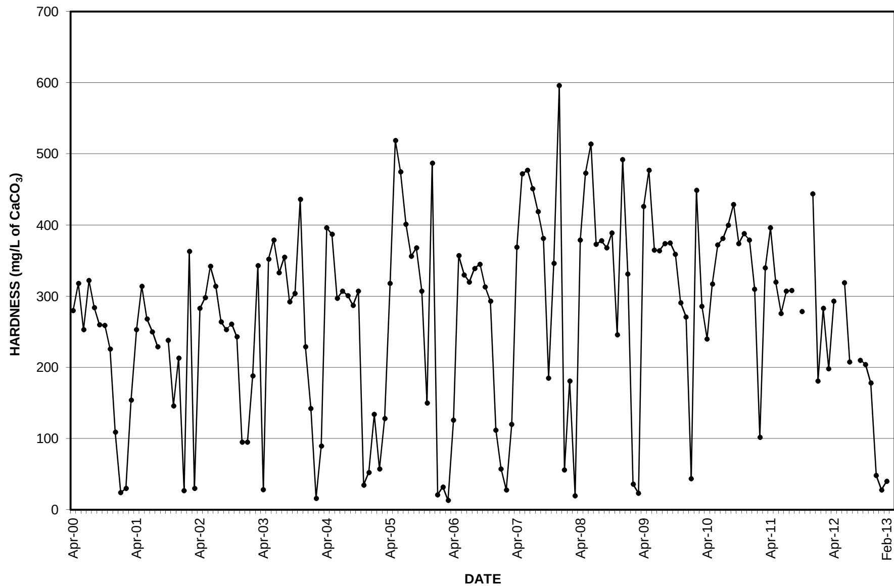
GRAPH 18 HARDNESS SETTLING POND 1
