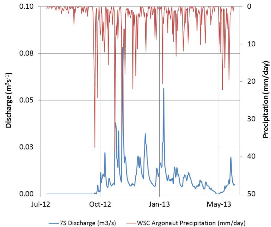
Figure A5.3: Daily discharge data for 7S hydrometric station. Precipitation data from the Water Survey of Canada rain gauge near Argonaut Bridge is shown on the secondary y-axis.
