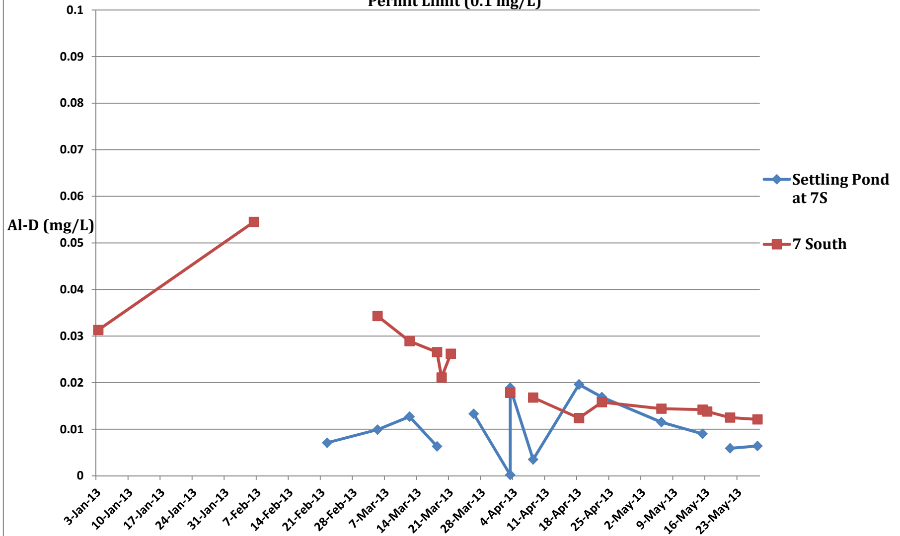
Graph 63 Dissolved Aluminum Settling Pond 7SSD vs 7S Permit Limit (0.1 mg/L)
