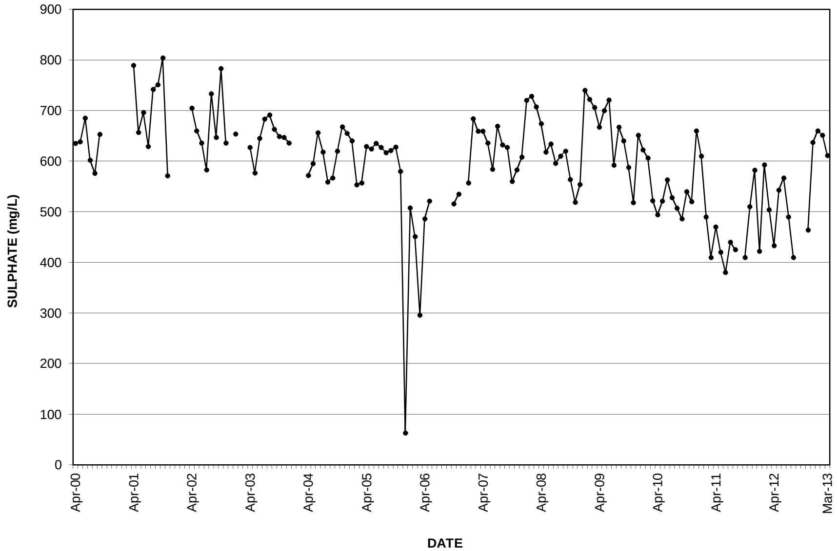
GRAPH 56 SULPHATE SEEP INTO LONG LAKE (LLS)
