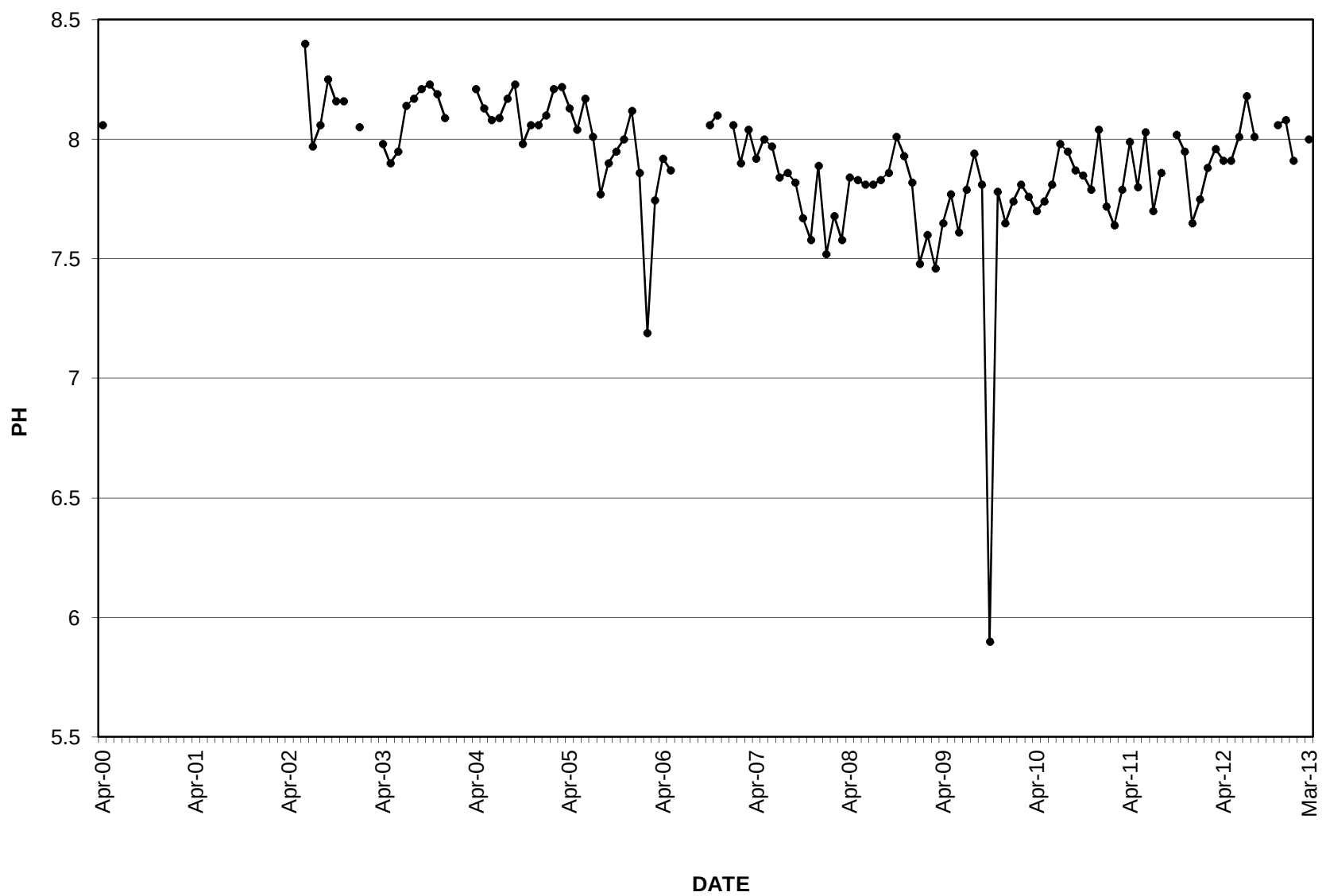
GRAPH 54 pH SEEP INTO LONG LAKE (LLS)
