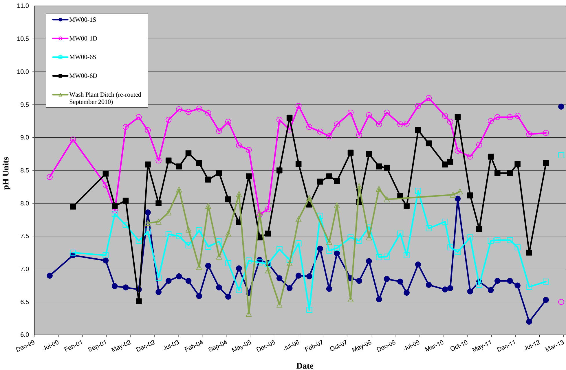
Graph 2: Compilation of Field Measured pH in Groundwater in the 2 North Area
