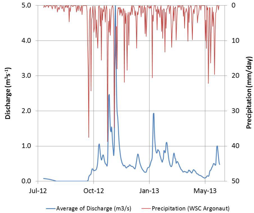
Figure A1.3: Daily discharge data for LLO hydrometric station. Precipitation data from the Water Survey of Canada rain gauge near Argonaut Bridge is shown on the secondary y-axis.
