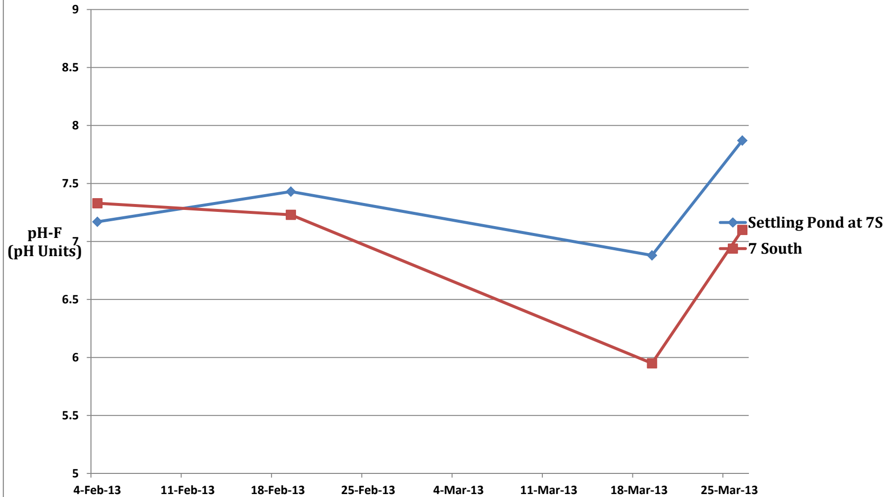
Graph 69 Field pH Settling Pond 7SSD vs 7S Permit Limit (6.0-8.0)
