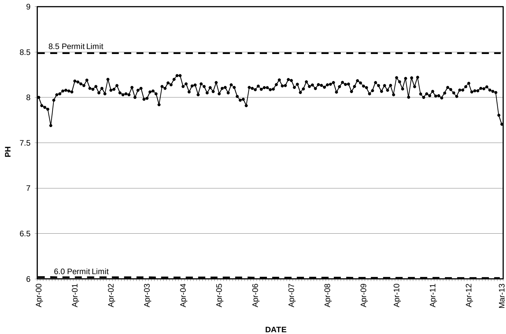
GRAPH 2 PH SETTLING POND 4
