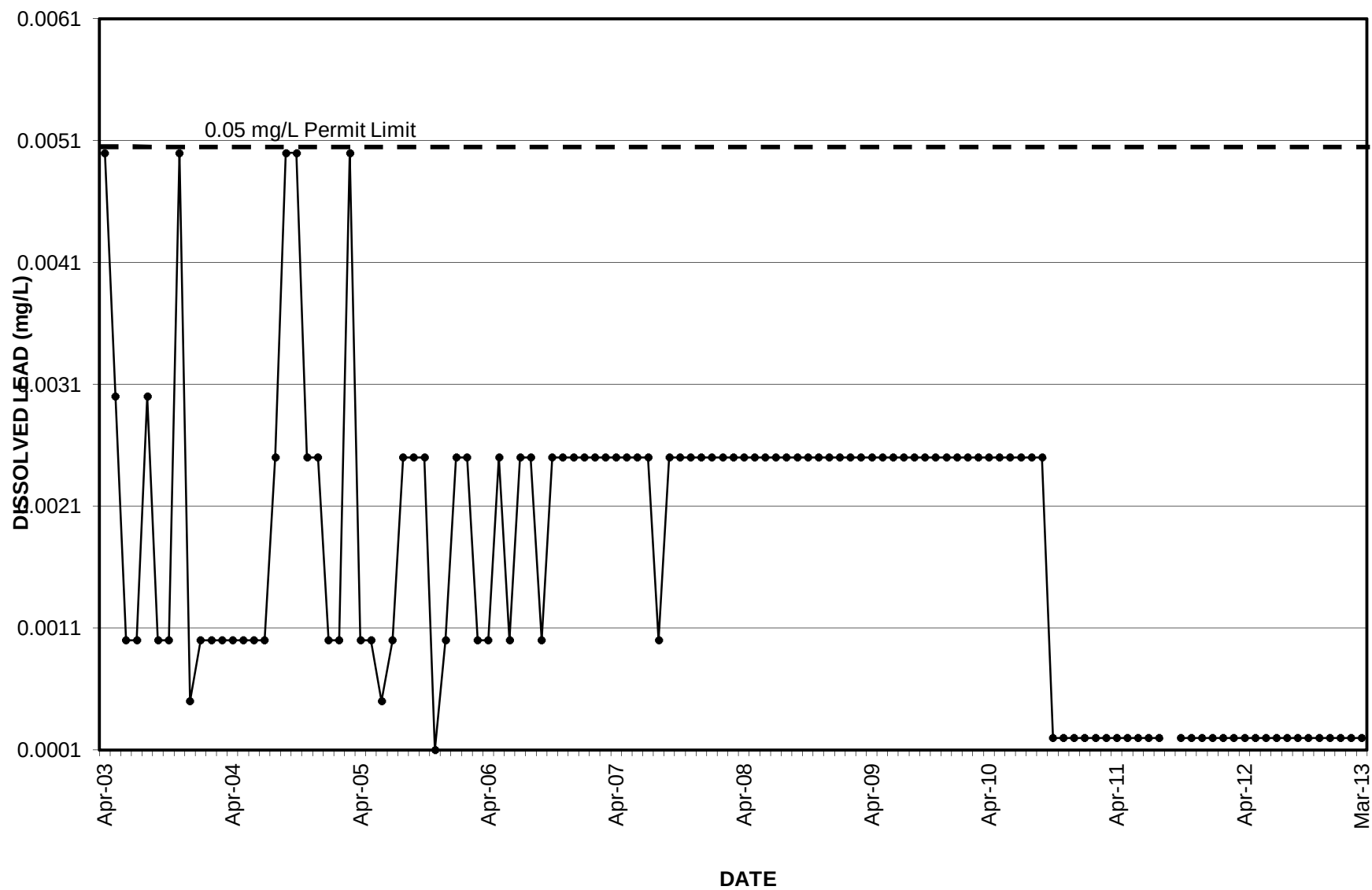
GRAPH 13 DISSOLVED LEAD SETTLING POND 4
