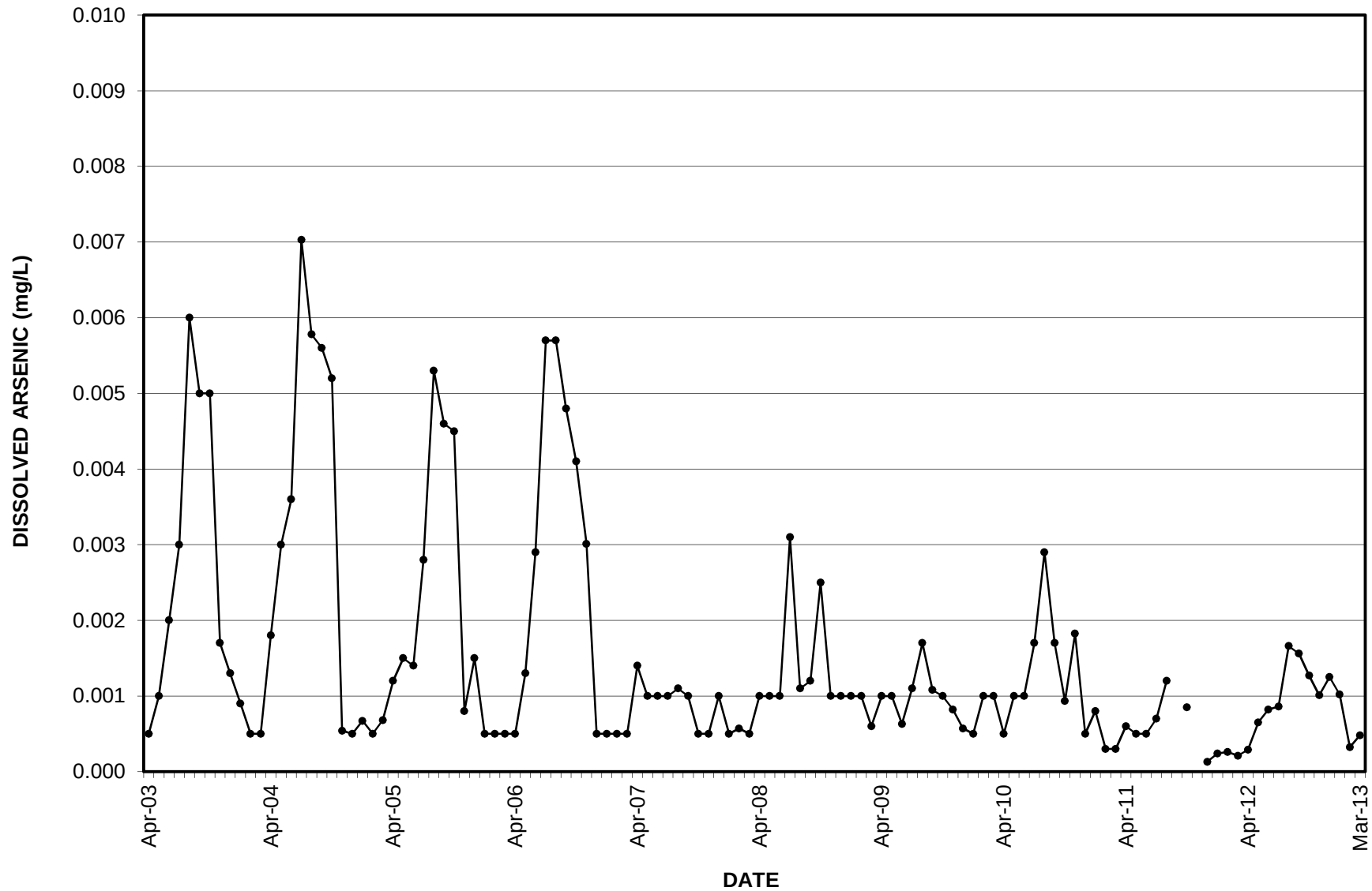
GRAPH 27 DISSOLVED ARSENIC SETTLING POND 1
