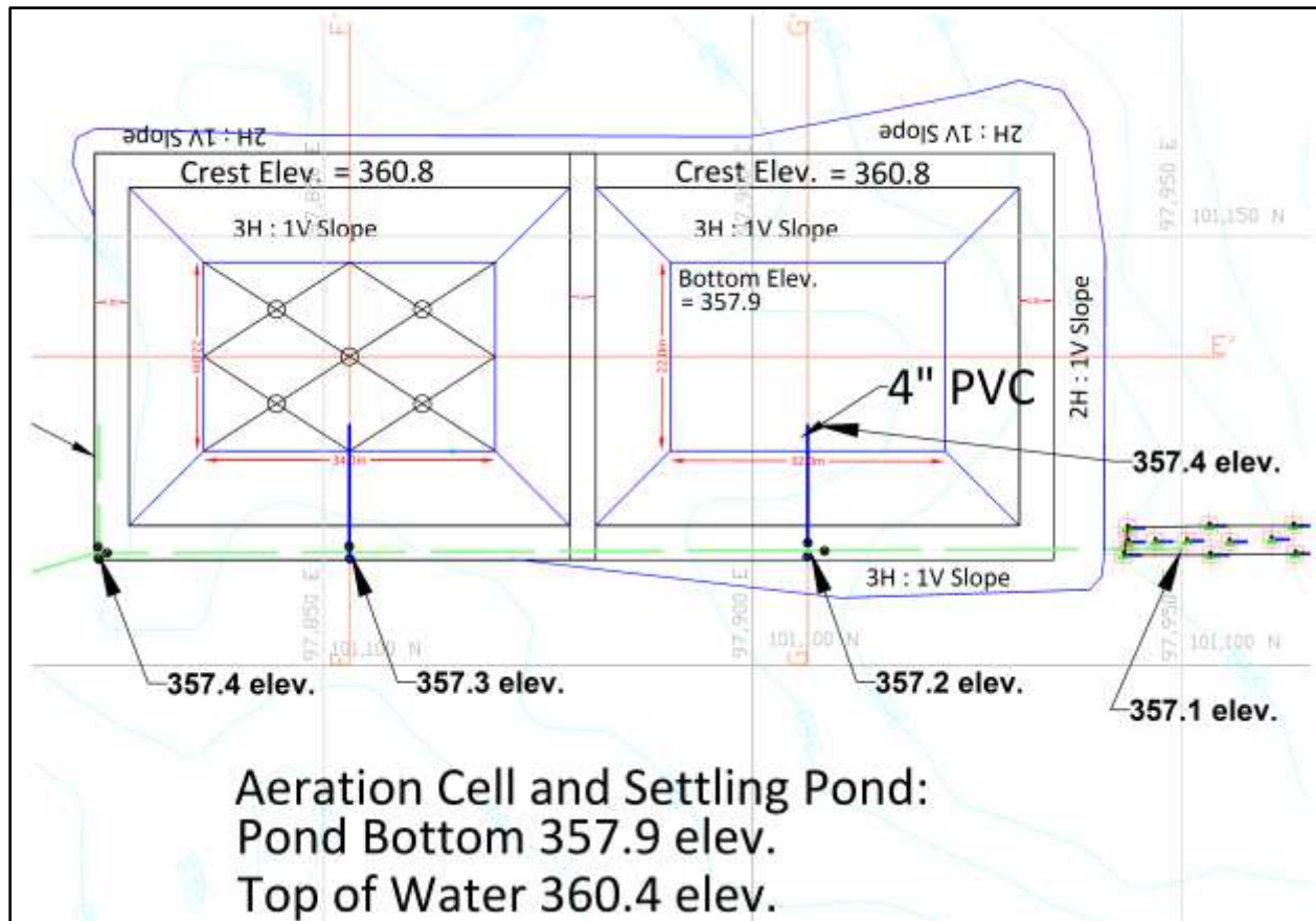
Figure 3: Aerobic Polishing System Construction Design – Layout
