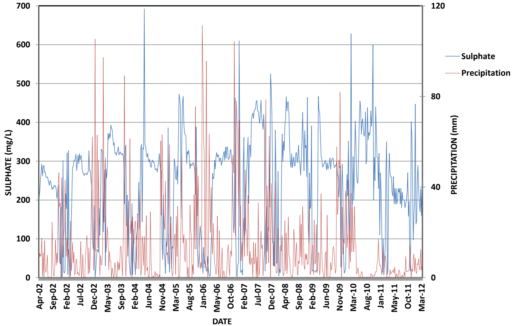
GRAPH 34 PRECIPITATION/SULPHATE SETTLING POND 1
