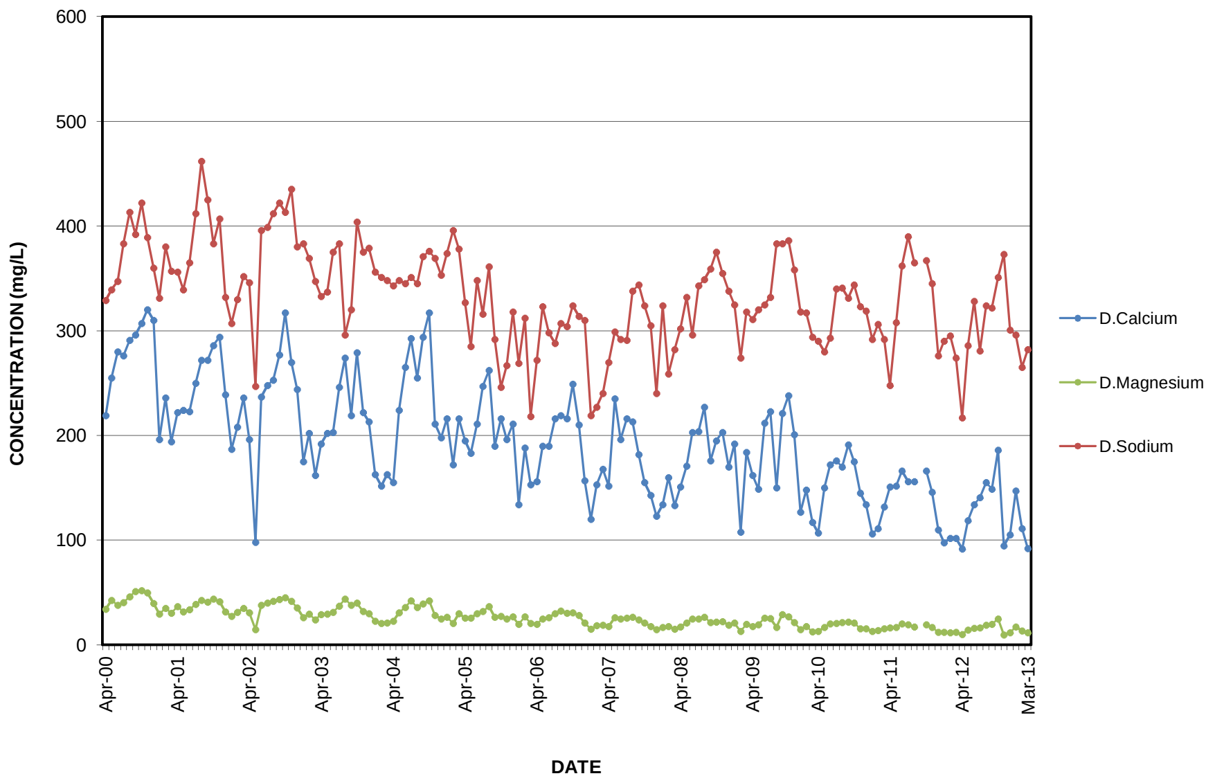
GRAPH 16 DISSOLVED CALCIUM/MAGNESIUM/SODIUM SETTLING POND 4
