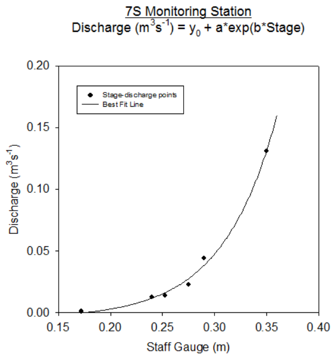
Figure A5.2: Stage-discharge relationship for the 7S hydrometric station. Values for y_0 , a , and b were determined to be -0.0048, 0.0002 and 19.1383 respectively.
