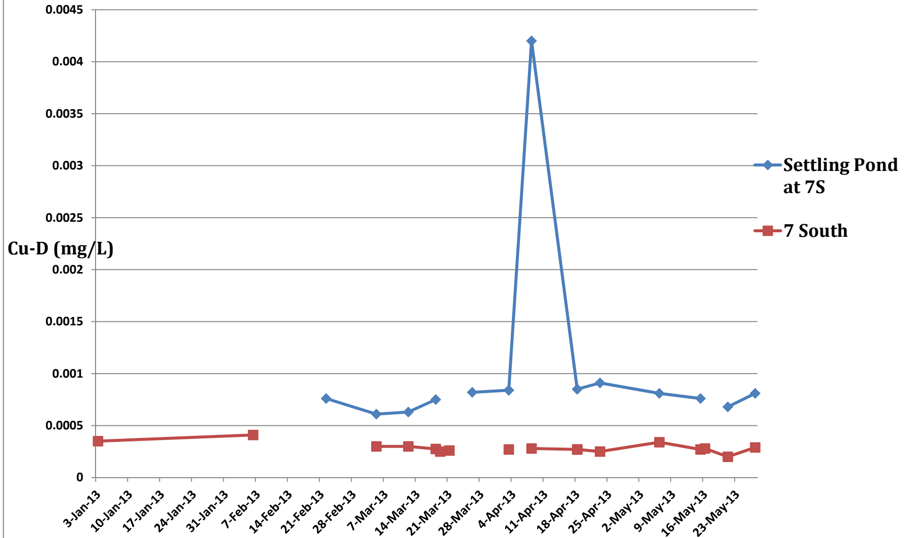
Graph 65 Dissolved Copper Settling Pond 7SSD vs 7S Permit Limit (0.014 mg/L)
