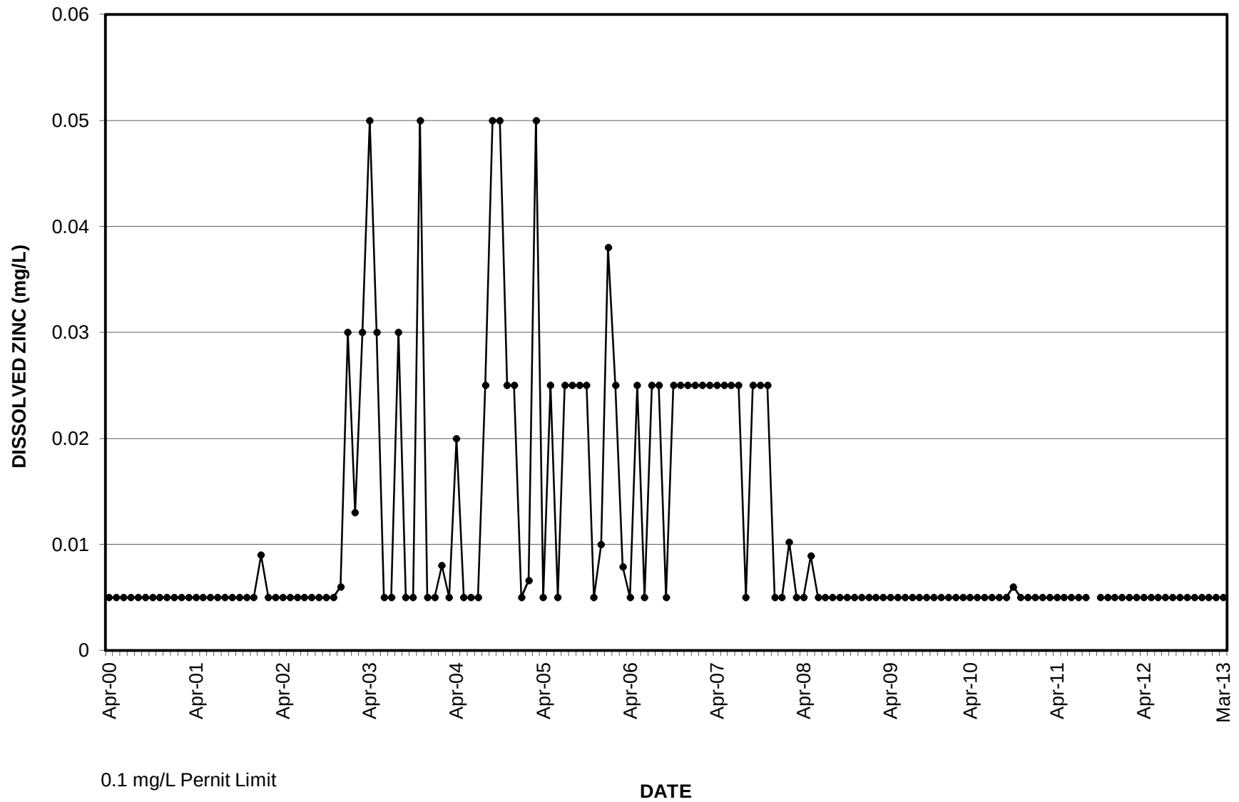
Graph 15 DISSOLVED ZINC Settling Pond 4
