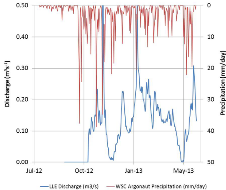
Figure A3.3: Daily discharge data for LLE hydrometric station. Precipitation data from the Water Survey of Canada rain gauge near Argonaut Bridge is shown on the secondary y-axis.
