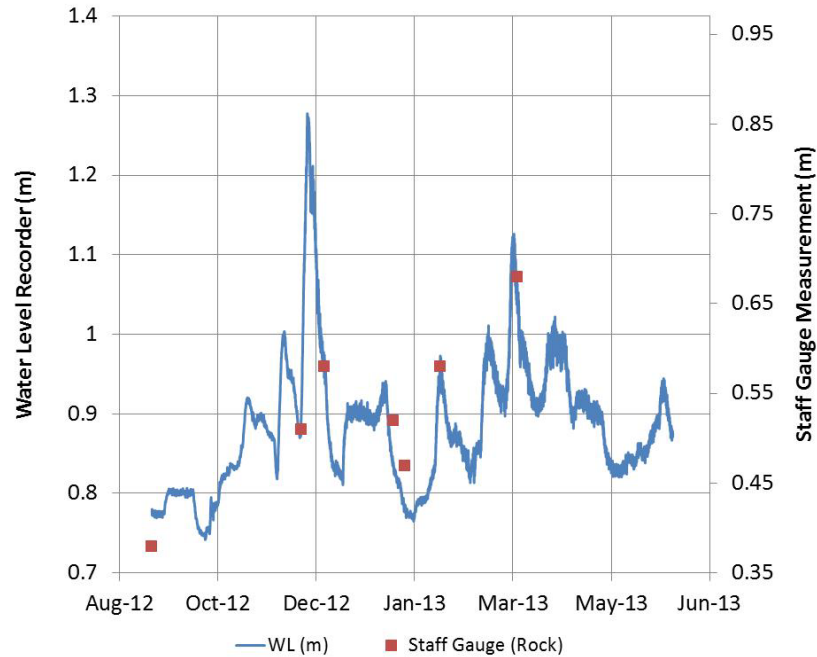
Figure A4.1: Relationship between continuous water level and spot measurements of stage at WB staff gauge for the period of record.
