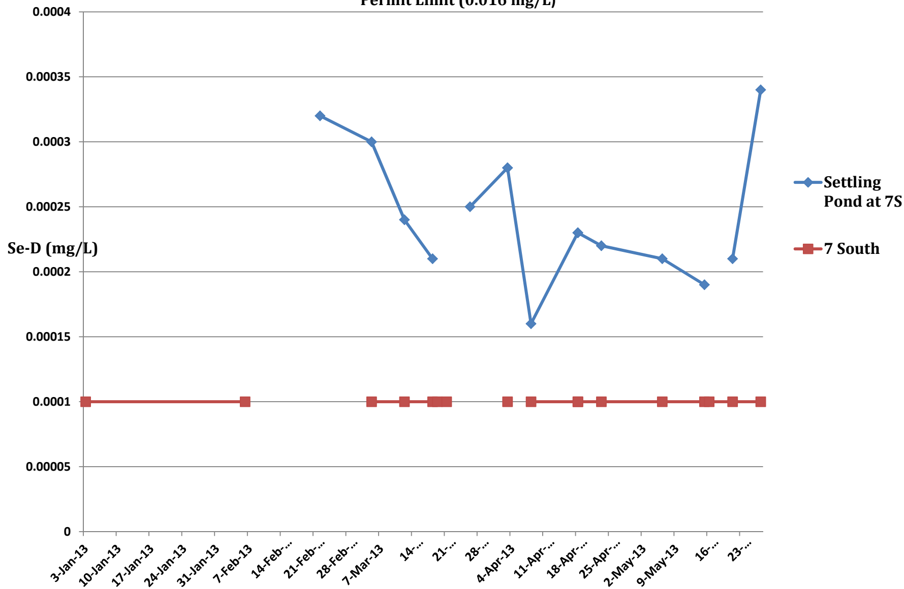
Graph 67 Dissolved Selenium Settling Pond 7SSD vs 7S Permit Limit (0.016 mg/L)
