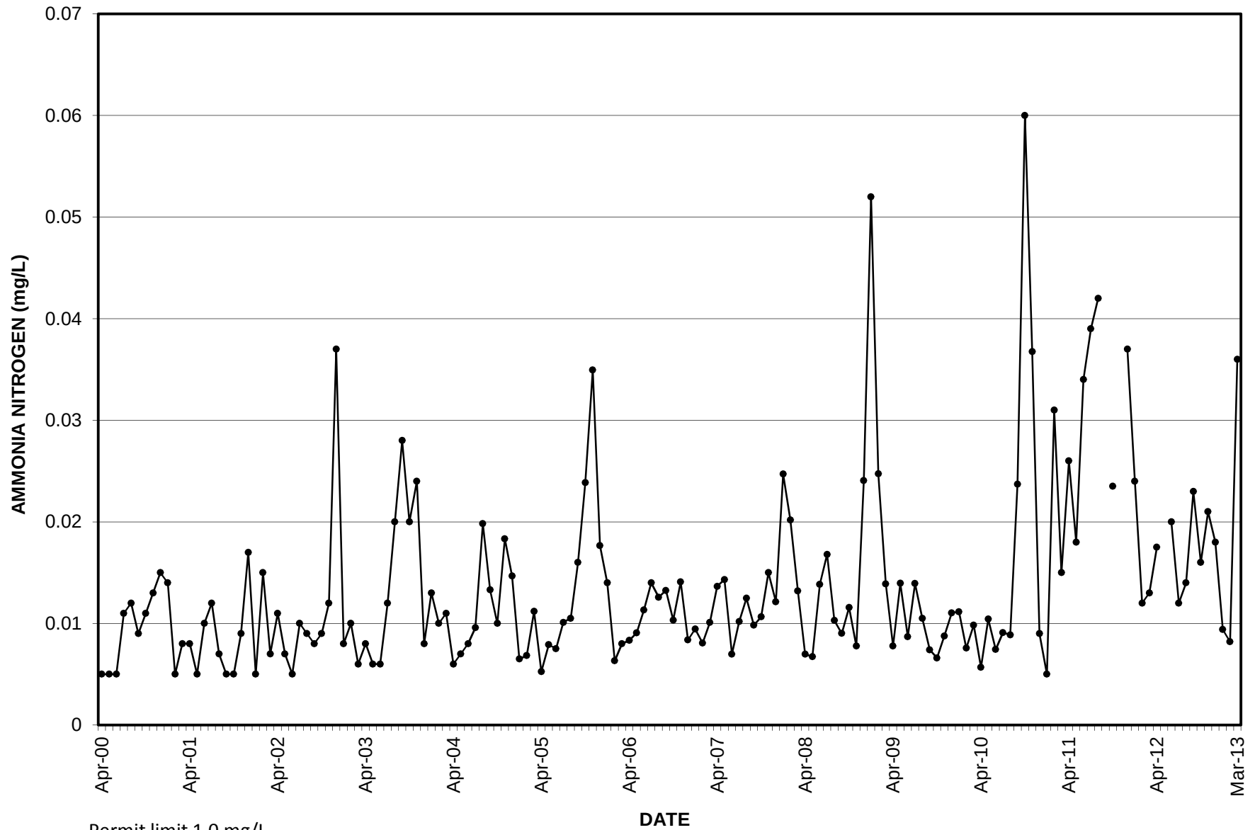
GRAPH 23 AMMONIA NITROGEN SETTLING POND 1
