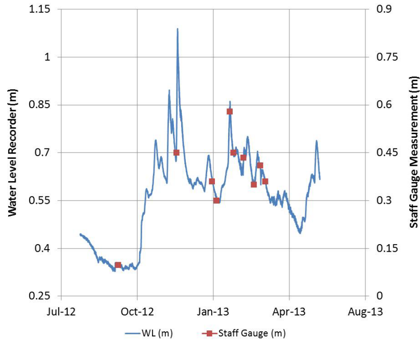
Figure A1.1: Relationship between continuous water level and spot measurements of stage at LLO staff gauges for the period of record.
