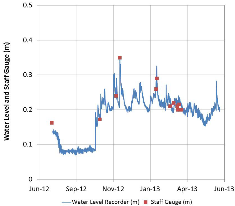
Figure A5.1: Relationship between continuous water level and spot measurements of stage at 7S staff gauge for the period of record.
