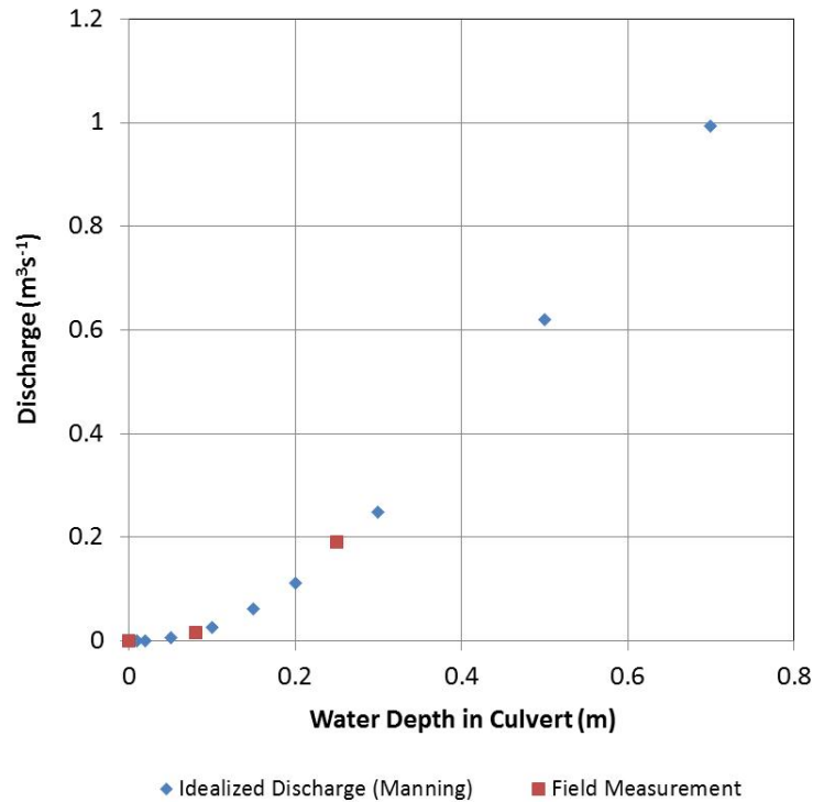
Figure A3.4: Comparison between idealized (Manning) estimates and field measurements of discharge at LLE culvert.
