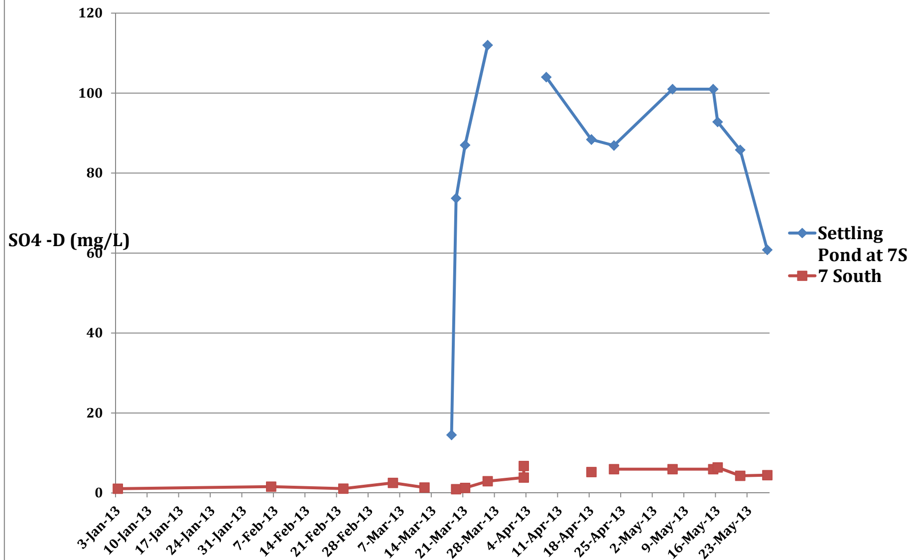
Graph 68 Dissolved Sulphate Settling Pond 7SSD vs 7S Permit Limit (500 mg/L)
