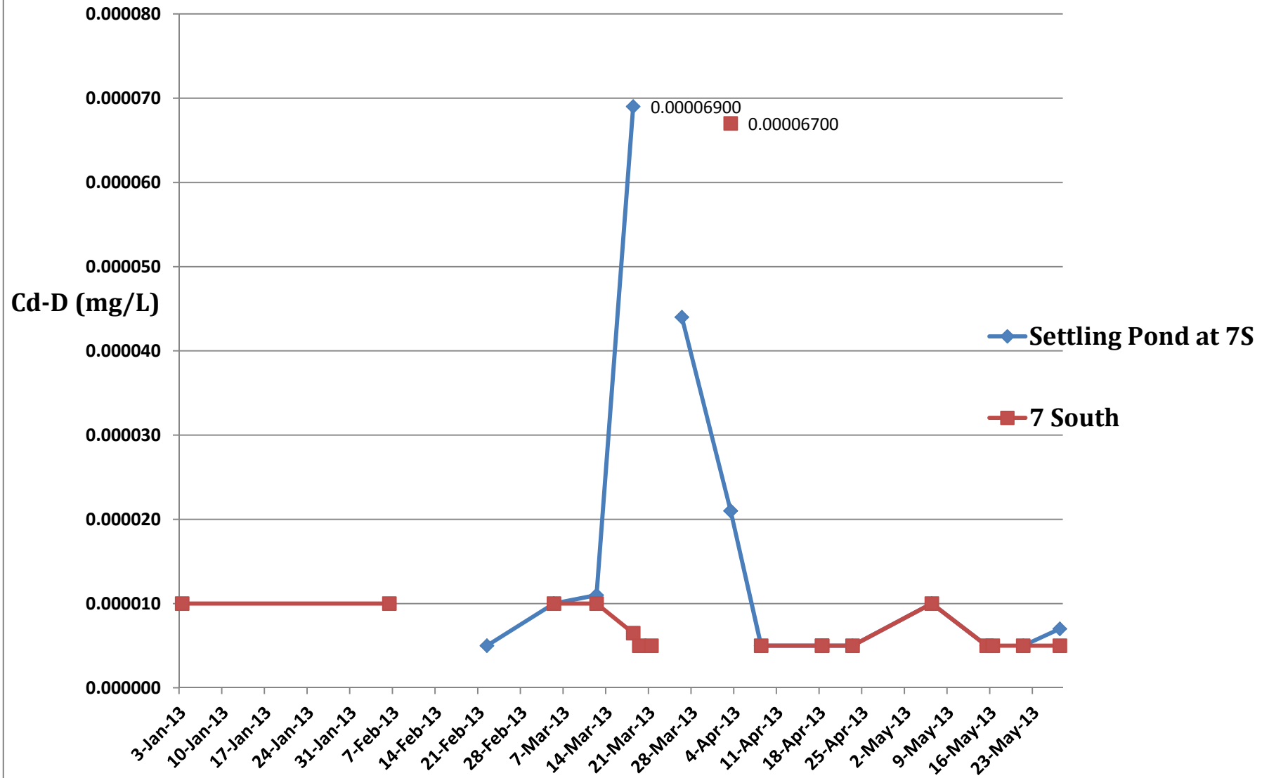
Graph 64 Dissolved Cadmium Settling POND 7SSD vs 7S Permit Limit (0.000045 mg/L)
