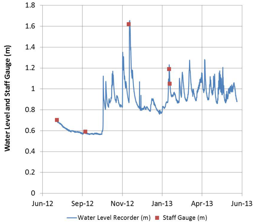
Figure A6.1: Relationship between continuous water level and spot measurements of stage at IR staff gauge for the period of record.
