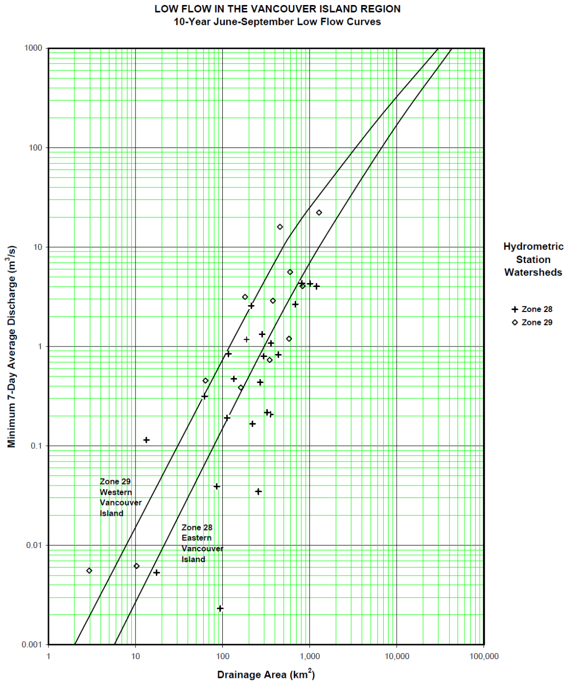
Figure B.2.1: Relationship between minimum 7-day average discharge and drainage area for Zone 28 (Eastern Vancouver Island) after Obedkoff (2003).
