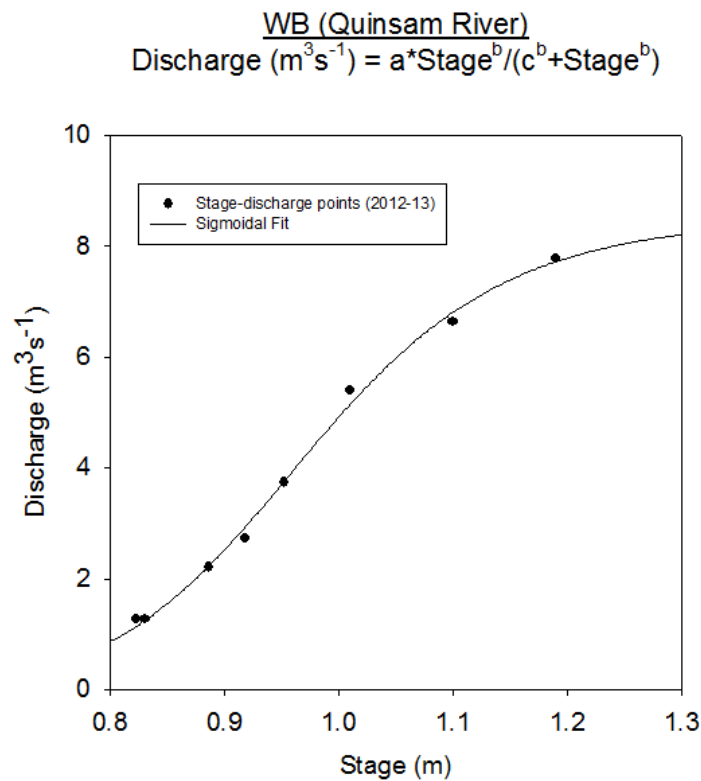
Figure A4.2: Stage-discharge relationship for the WB hydrometric station. Values for a, b, and c were determined to be 8.53, 11.15 and 0.97 respectively.
