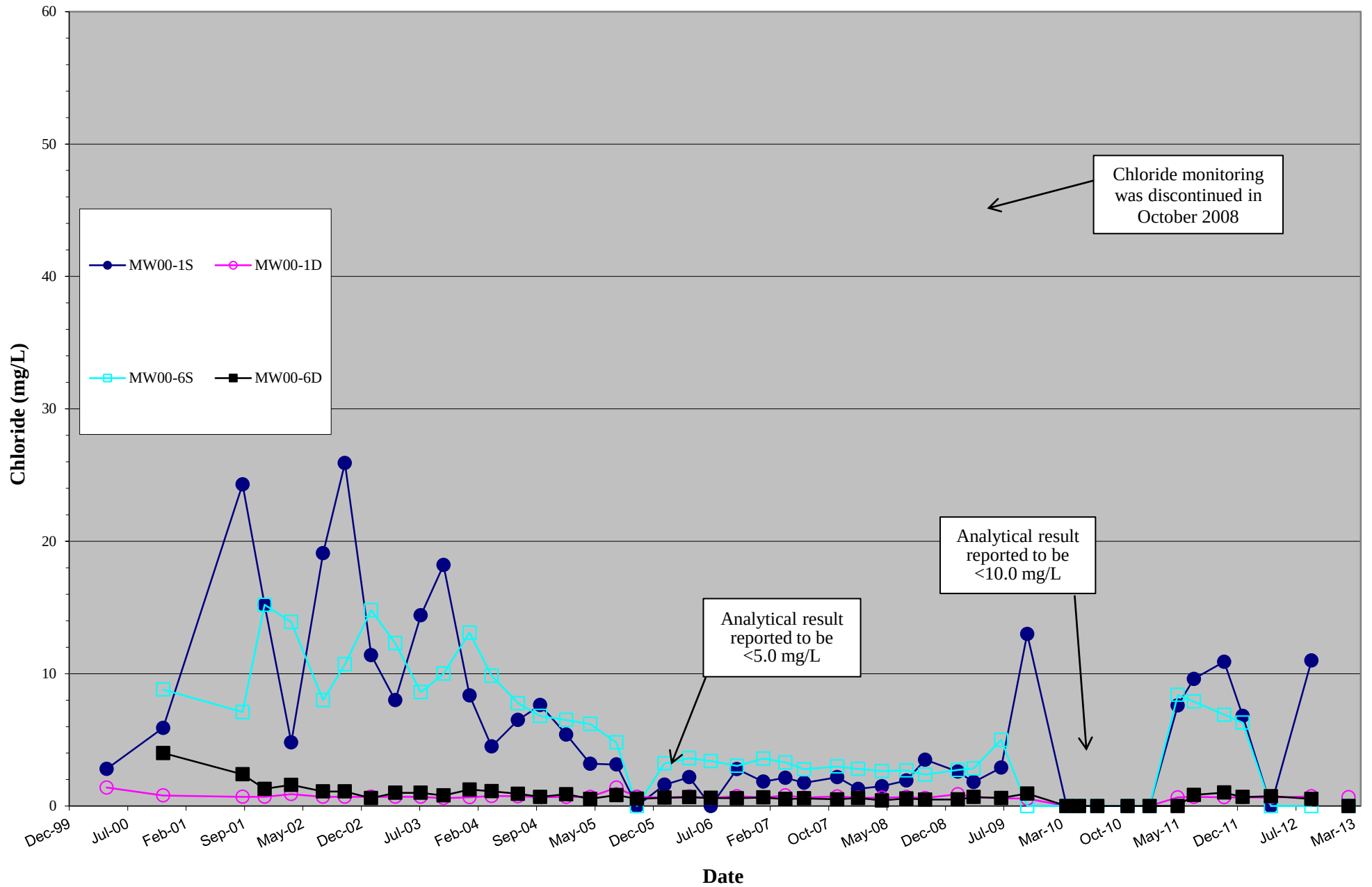
Graph 3: Compilation of Groundwater Chloride Concentrations in the 2 North Area
