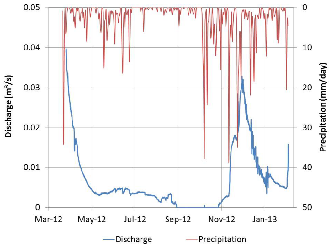
Figure A2.3: Daily discharge data for LLS hydrometric station. Precipitation data from the Water Survey of Canada rain gauge near Argonaut Bridge is shown on the secondary y-axis.
