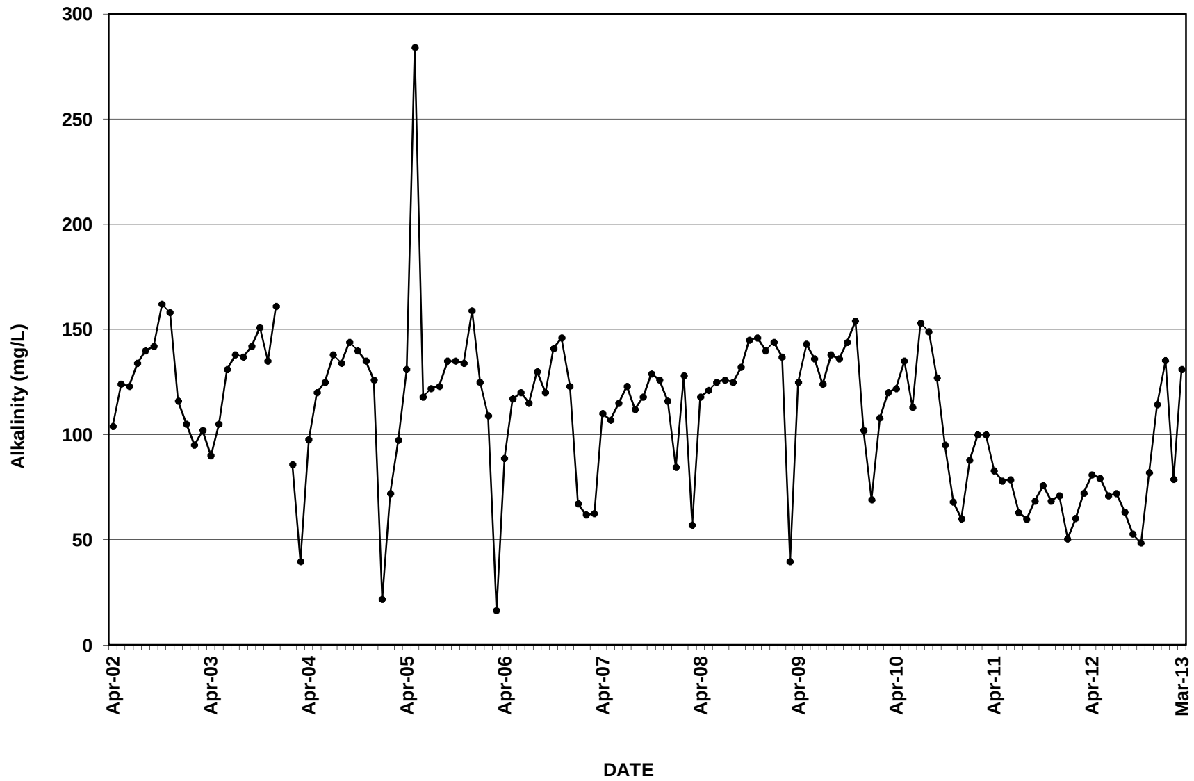
GRAPH 39 Alkalinity 3 SOUTH PIT
