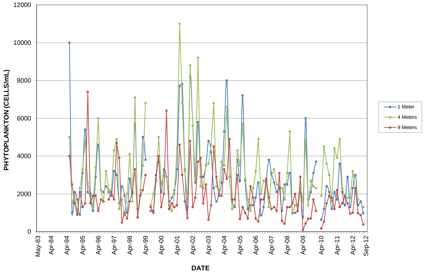
GRAPH 51 LONG LAKE PHYTOPLANKTON ABUNDANCE
