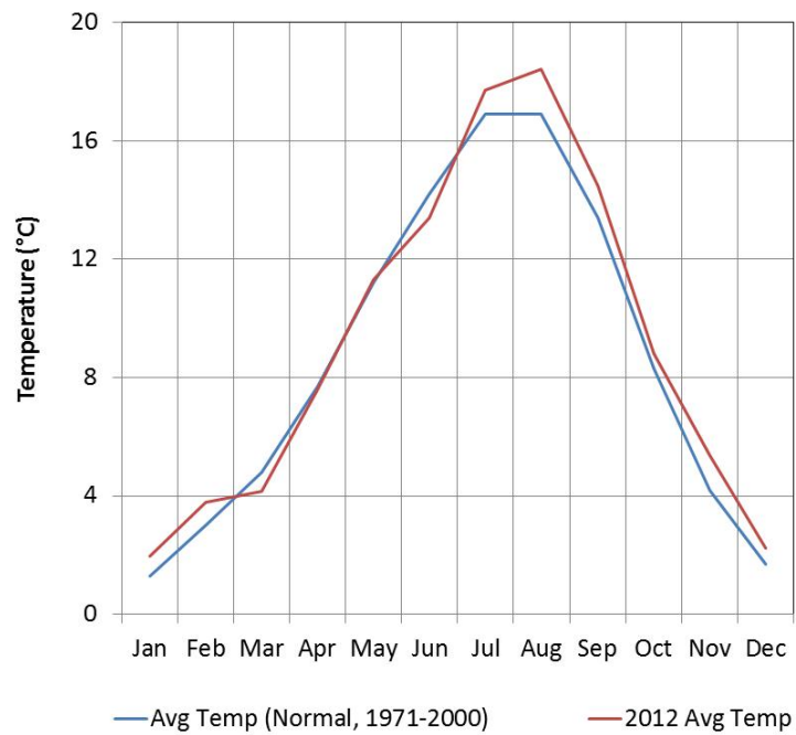
Figure 2: Comparison of monthly air temperature data for Campbell River. In the plot, 2012 data are compared to normal conditions for the station.
