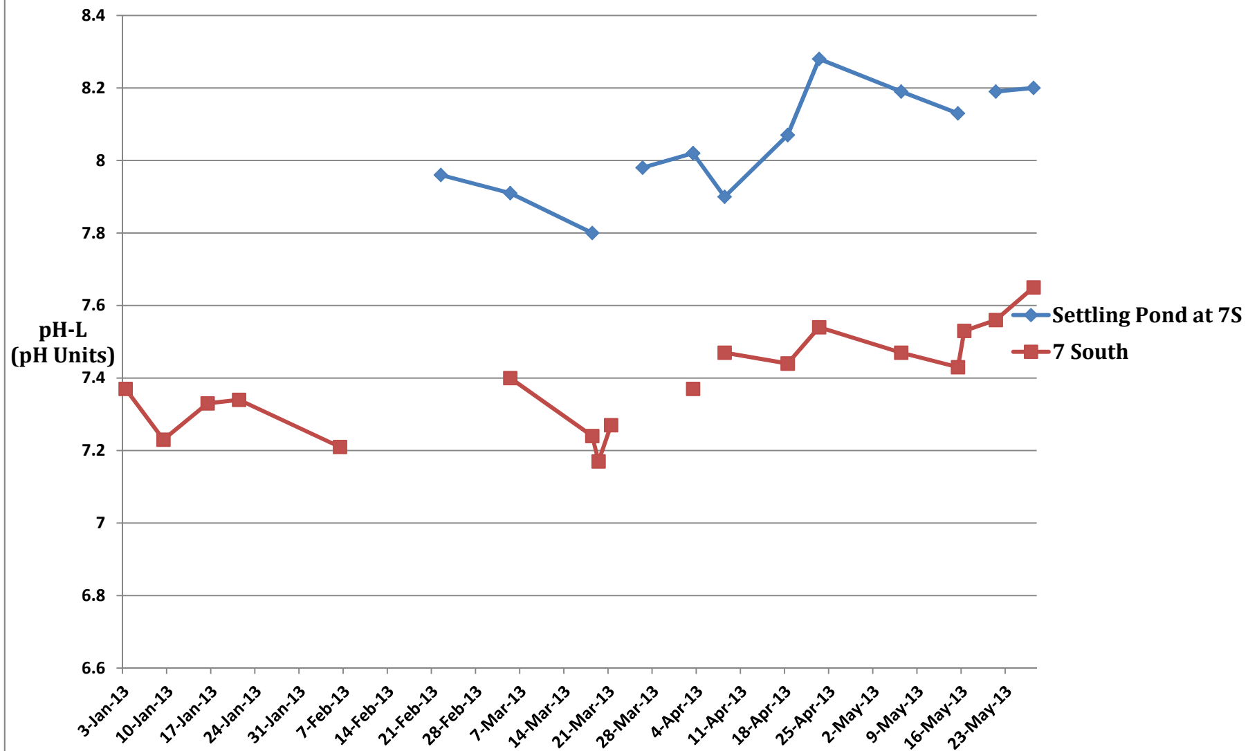
Graph 70 Lab pH Settling Pond 7SSD vs 7S Permit Limit (6.0-8.0)
