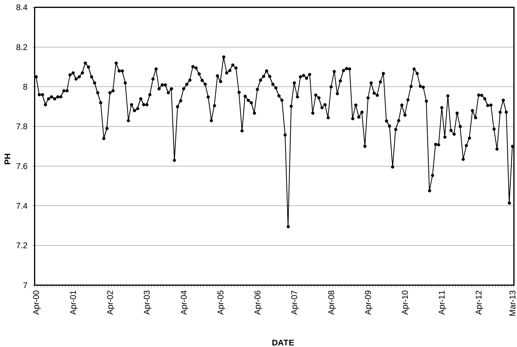
GRAPH 38 PH 3 SOUTH PIT
