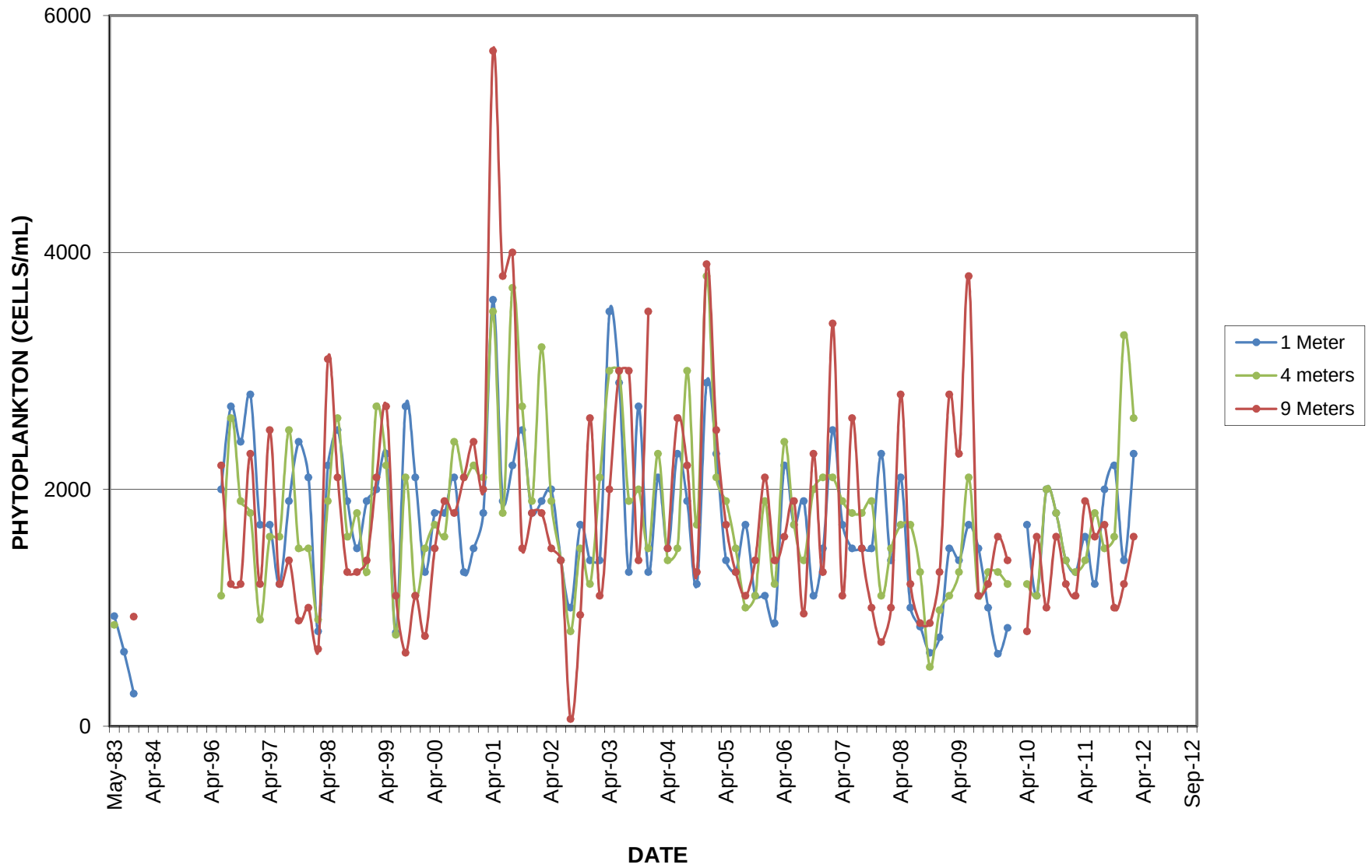
GRAPH 45 MIDDLE QUINSAM LAKE PHYTOPLANKTON ABUNDANCE
