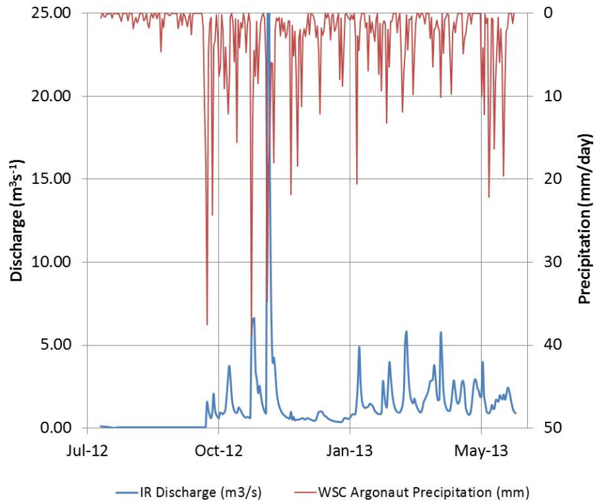
Figure A6.3: Daily discharge data for IR hydrometric station. Precipitation data from the Water Survey of Canada rain gauge near Argonaut Bridge is shown on the secondary y-axis.
