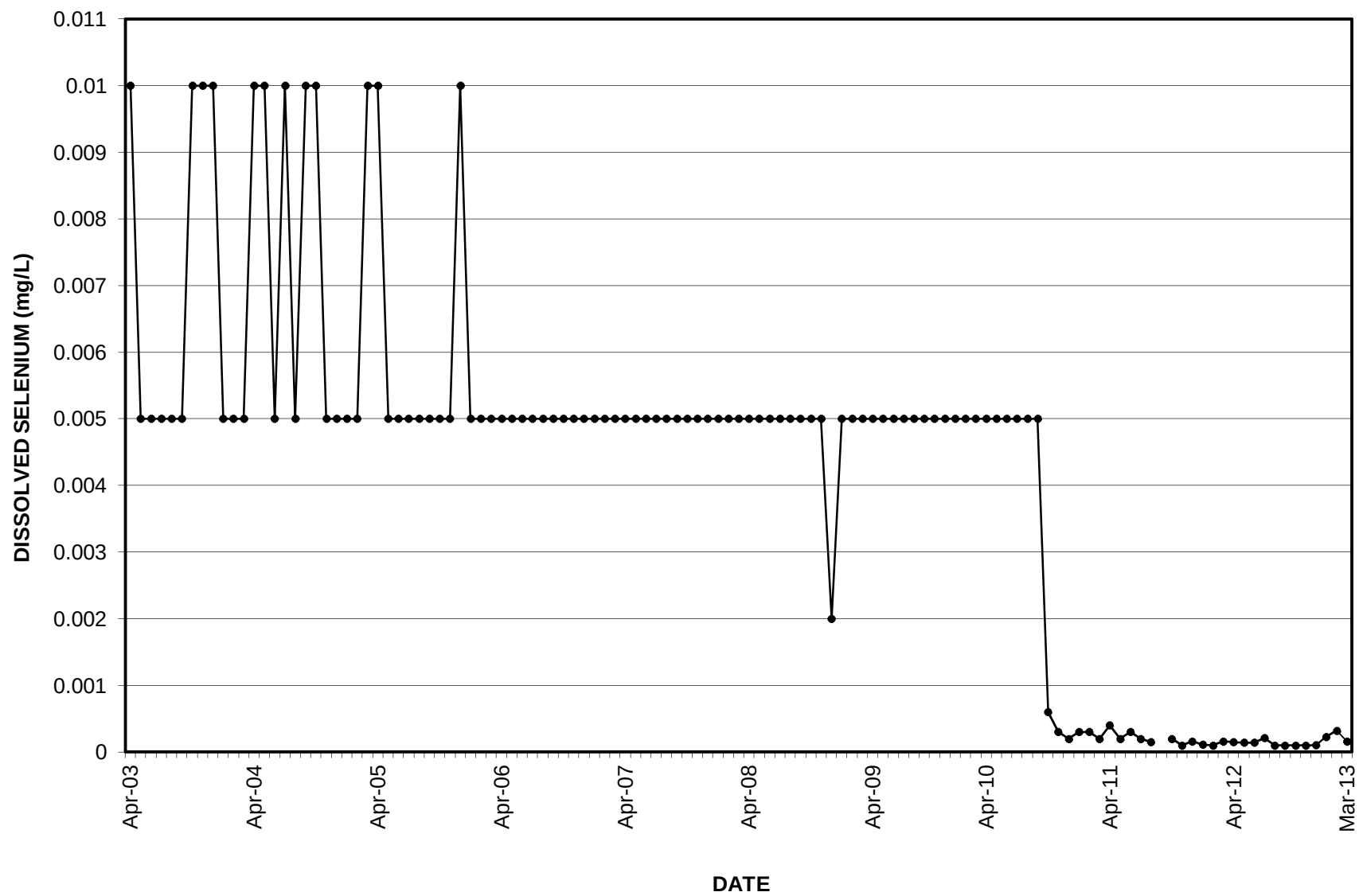
GRAPH 14 DISSOLVED SELENIUM SETTLING POND 4
