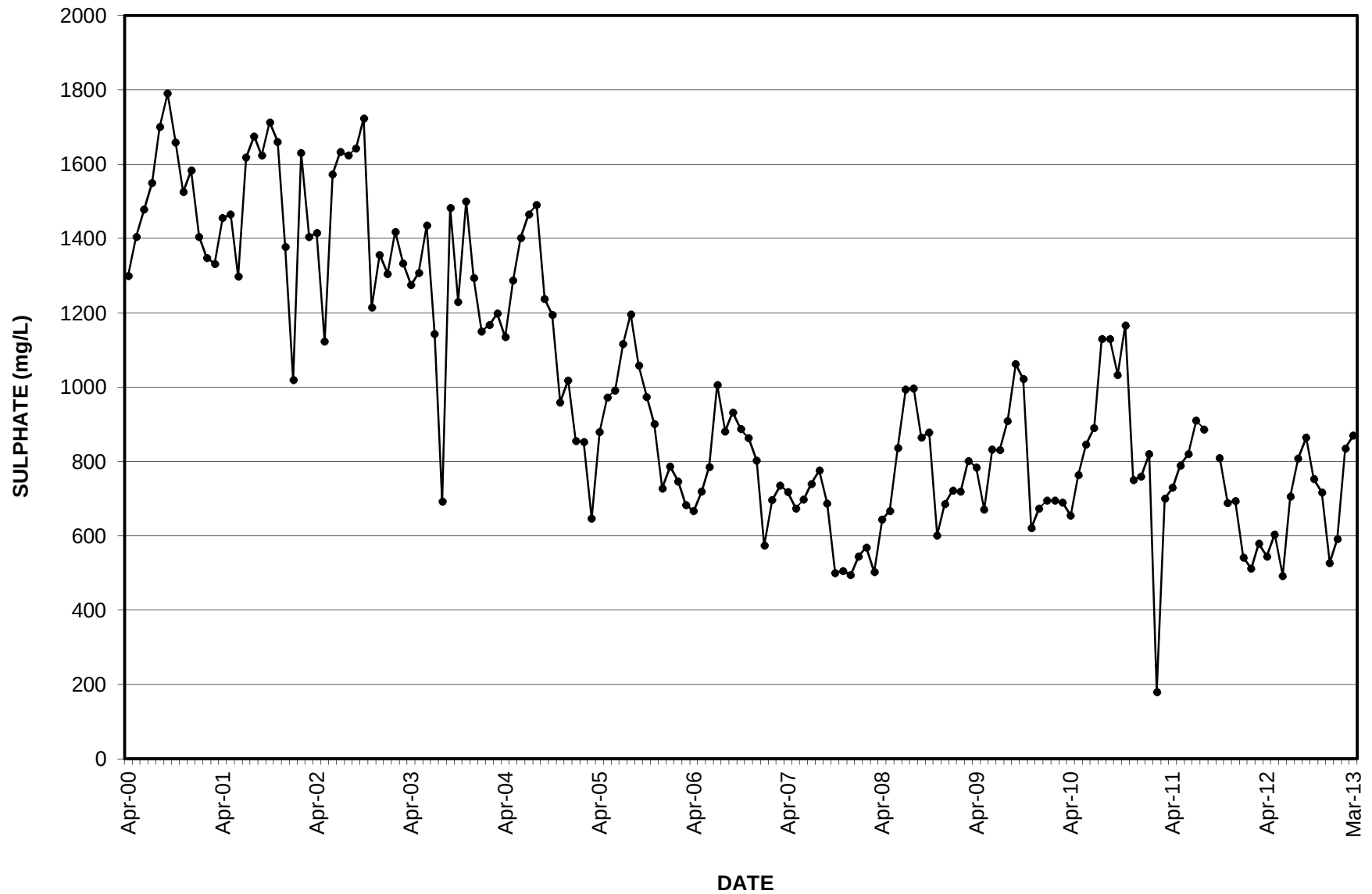
GRAPH 37 SULPHATE NORTH PIT SUMP (WP)
