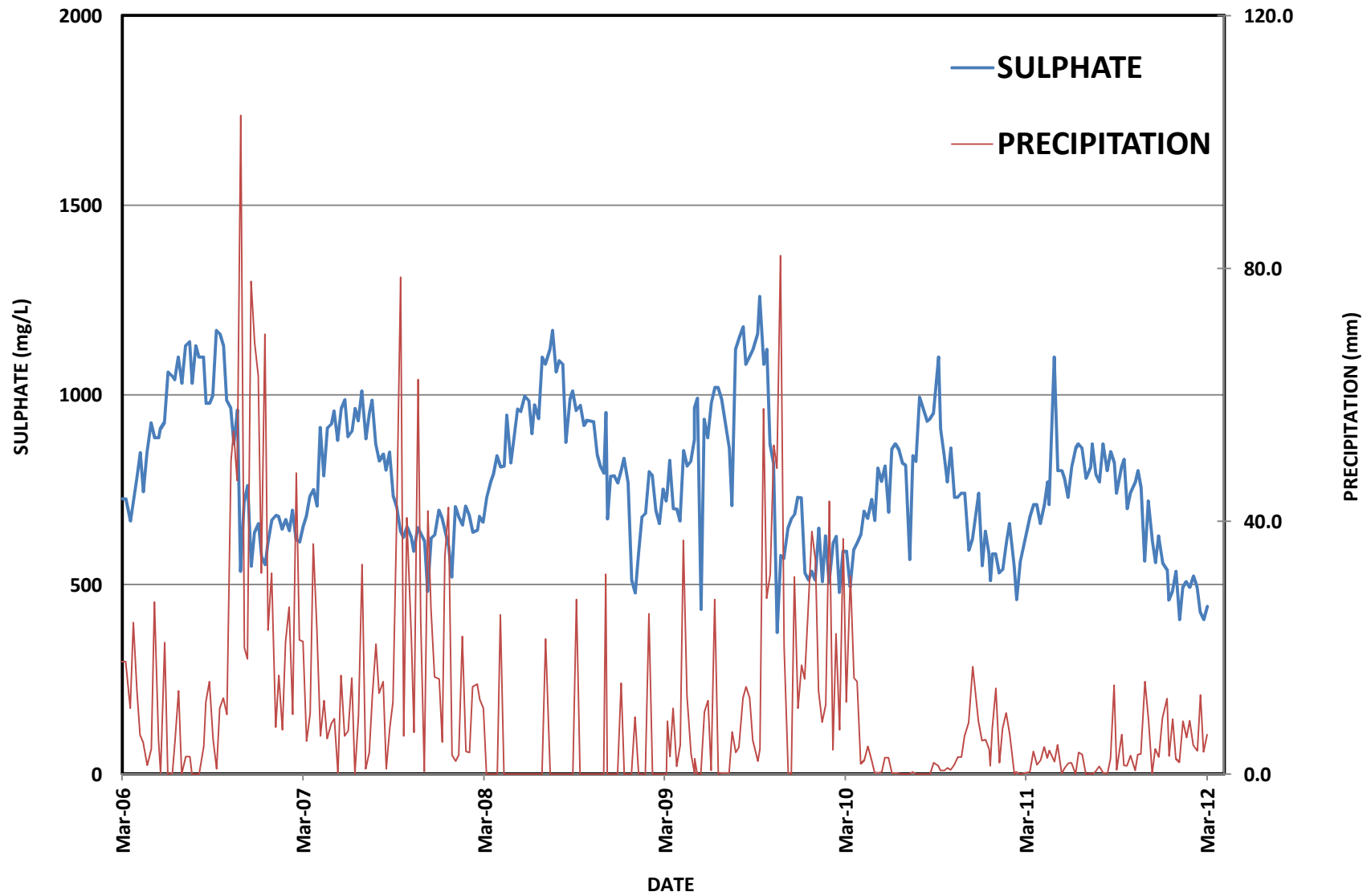
GRAPH 17 PRECIPITATION/SULPHATE SETTLING POND 4
