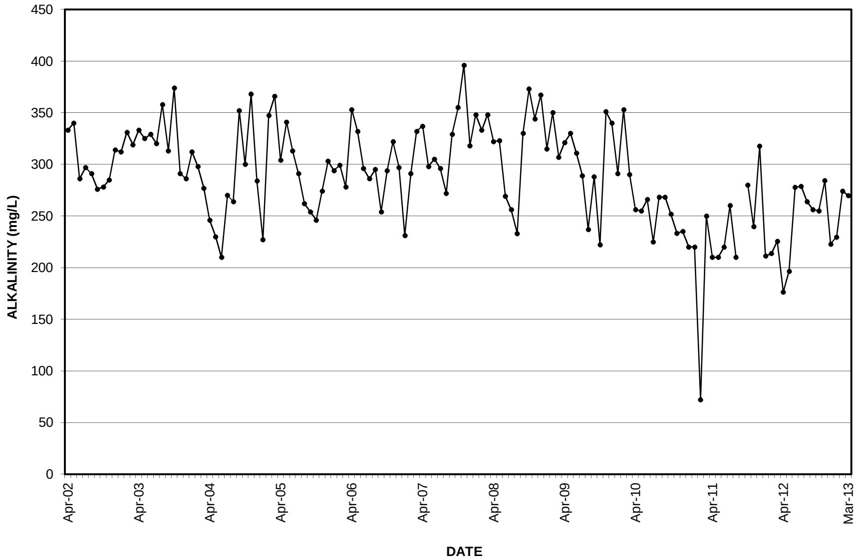
GRAPH 36 ALKALINITY NORTH PIT SUMP (WP)
