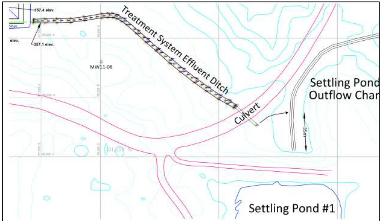
Figure 4: Settling Pond Effluent Channel Construction Design – Layout
