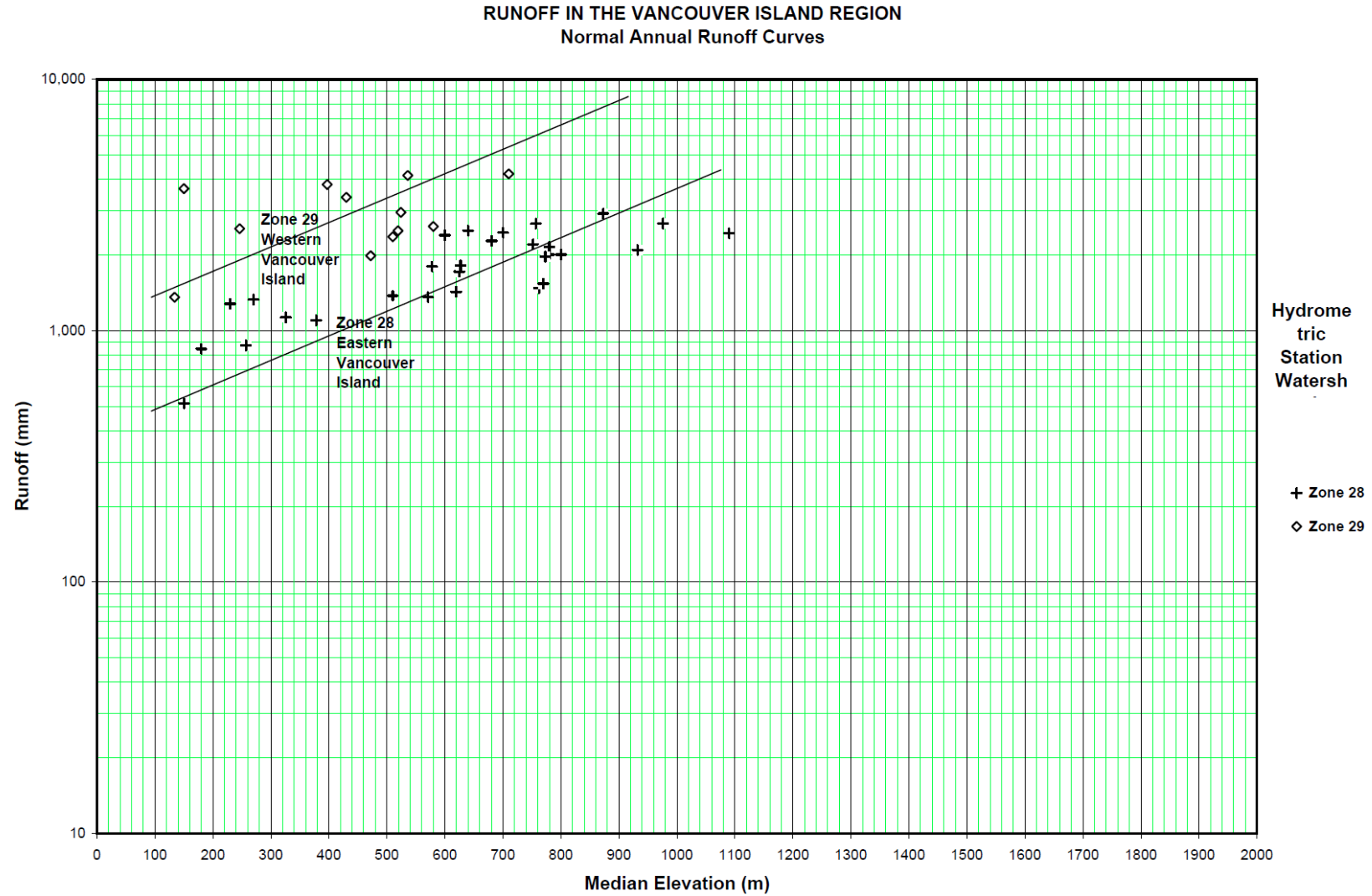
Figure B2.1: Relationship between annual runoff and watershed elevation for Zone 28 (Eastern Vancouver Island) after Obedkoff (2003).
