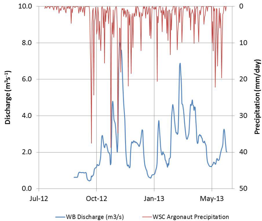
Figure A4.3: Daily discharge data for WB hydrometric station. Precipitation data from the Water Survey of Canada rain gauge near Argonaut Bridge is shown on the secondary y-axis.
