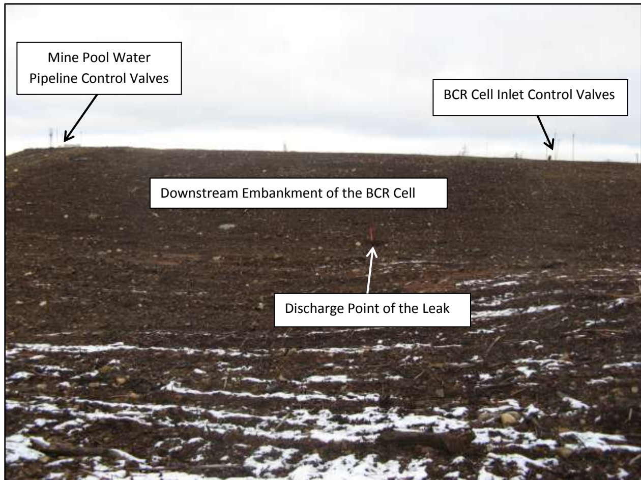
Photograph 2: Leak from the BCR Cell
