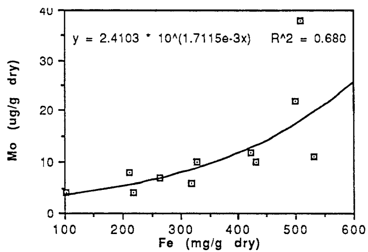
Figure 40: Mo as a function of Fe: northern Cascade Mountains.
