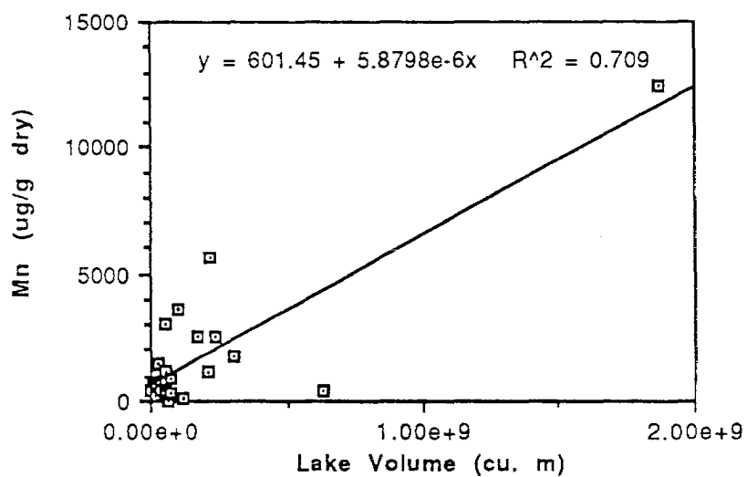
Figure 12: Mn as a function of lake volume: northern Omineca Belt.
