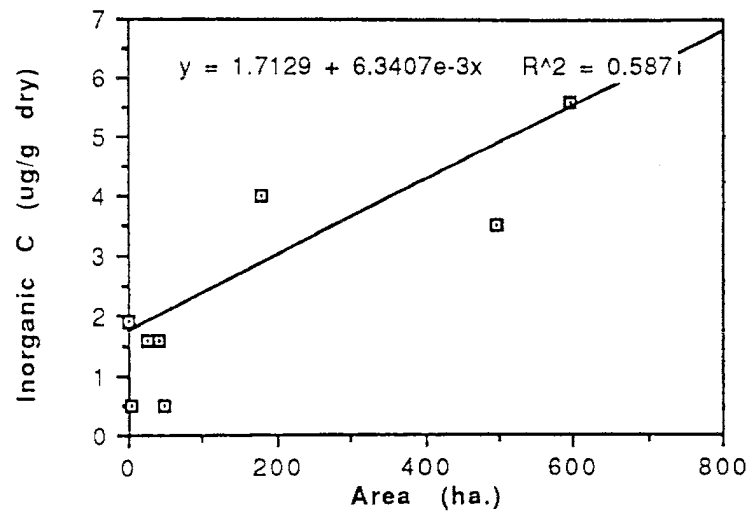
Figure 1: Inorganic C as a function of surface area: northern Insular Belt.
