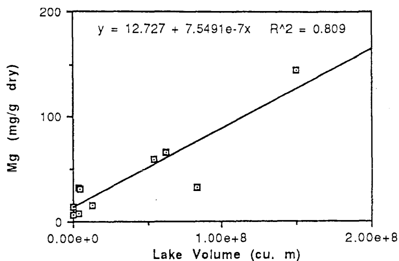
Figure 11: Mg as a function of lake volume: northern Insular Belt.
