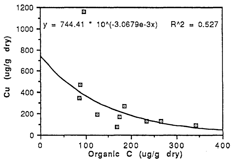
Figure 4: Cu as a function of organic C: northern Insular Belt.
