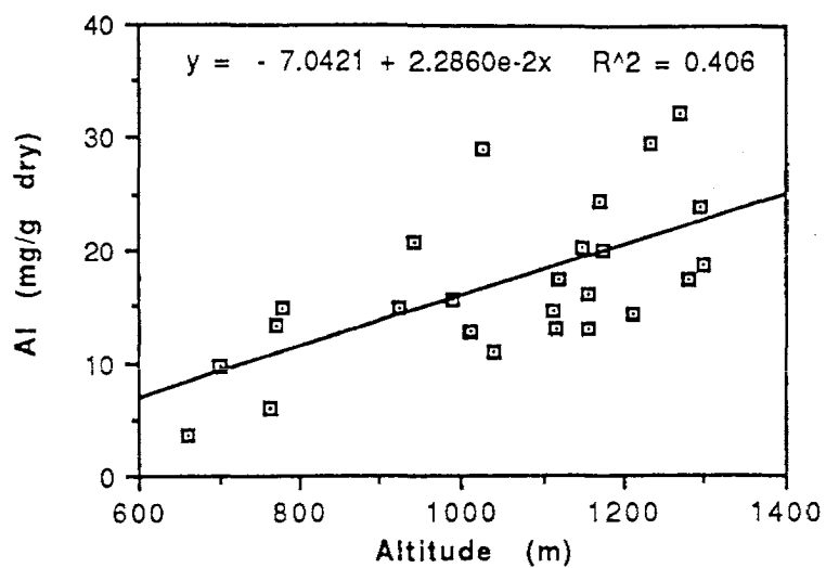
Figure 1: Al as a function of altitude: northern Omineca Belt.
