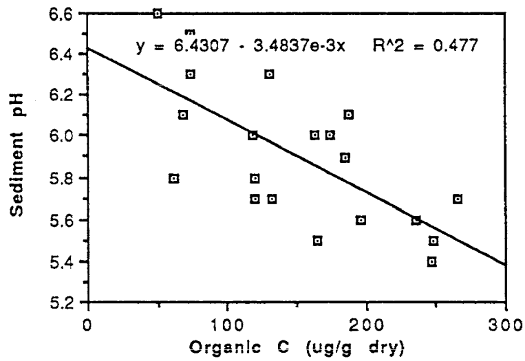
Figure 26: Sediment pH as a function of organic C: Insular Belt.
