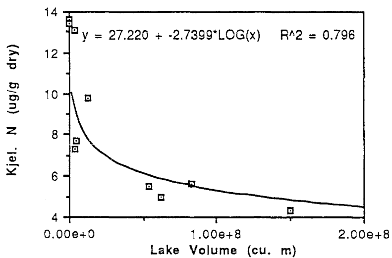
Figure 14: Kjeldahl N as a function of lake volume: northern Insular Belt.
