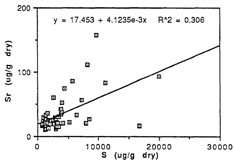
Figure 8: Sr as a function of S: southern Insular Belt.
