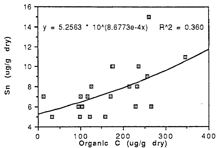
Figure 21: Sn as a function of organic C: Alberta Plateau.
