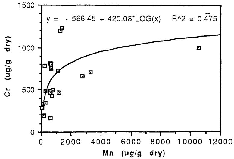
Figure 13: Cr as a function of Mn: central Omineca Belt.
