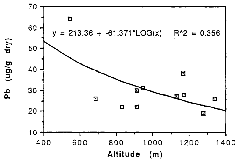
Figure 6: Pb as a function of altitude: northern Rocky Mountains.
