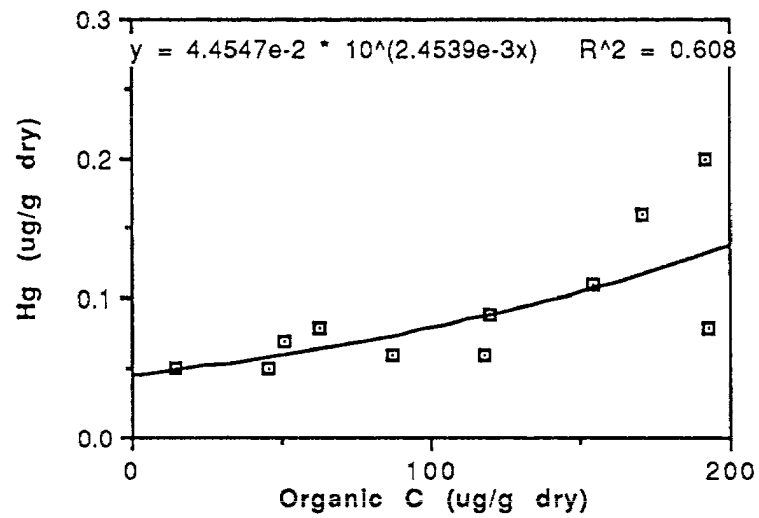
Figure 8: Hg as a function of organic C: northern Cascade Mountains.
