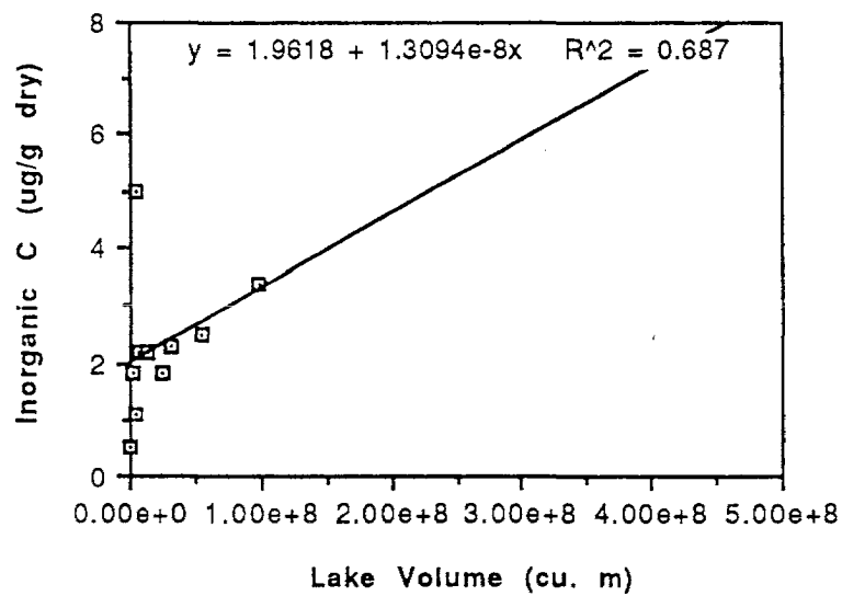
Figure 2: Inorganic C as a function of lake volume: northern Cascade Mountains.
