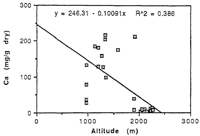
Figure 5: Ca as a function of altitude: southern Rocky Mountains.
