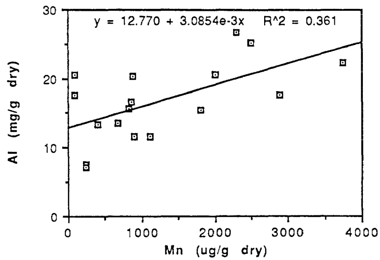
Figure 1: Al as a function of Mn: northern Interior Plateau.
