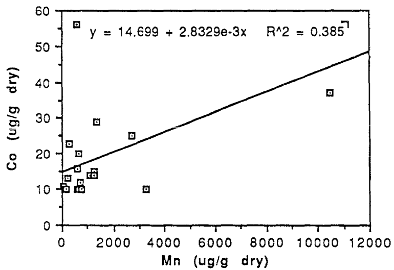
Figure 10: Co as a function of Mn: central Omineca Belt.
