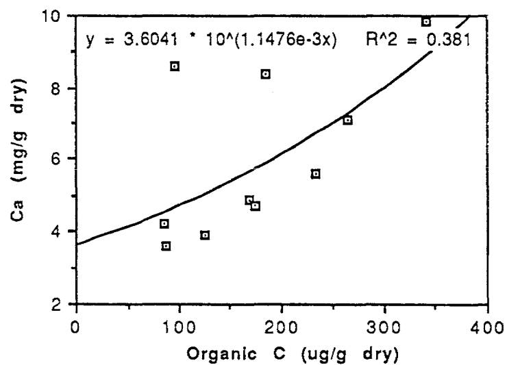
Figure 2: Ca as a function of organic C: northern Insular Belt.
