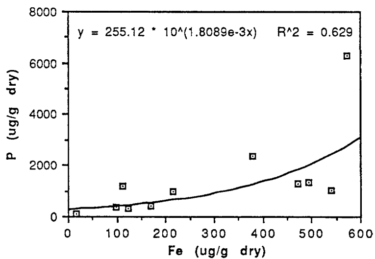
Figure 48: P as a function of Fe: northern Rocky Mountains.
