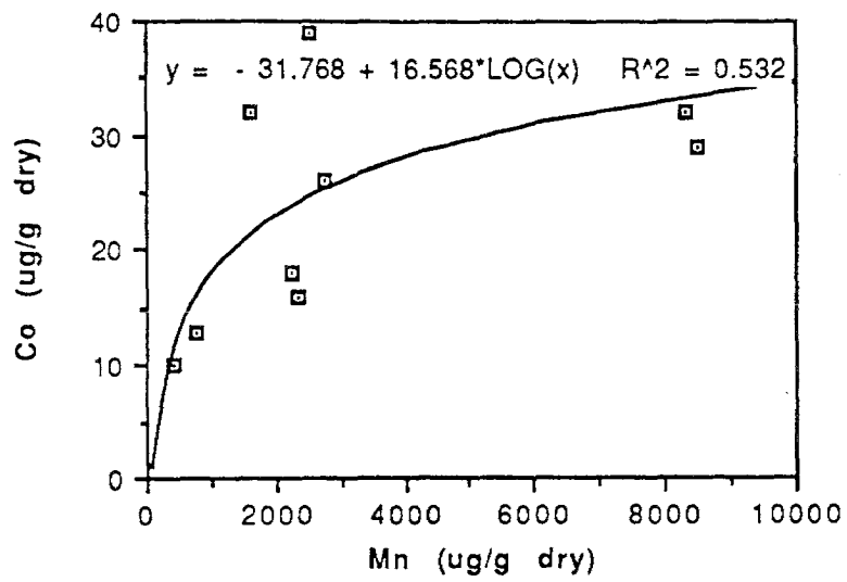
Figure 9: Co as a function of Mn: northern Insular Belt.
