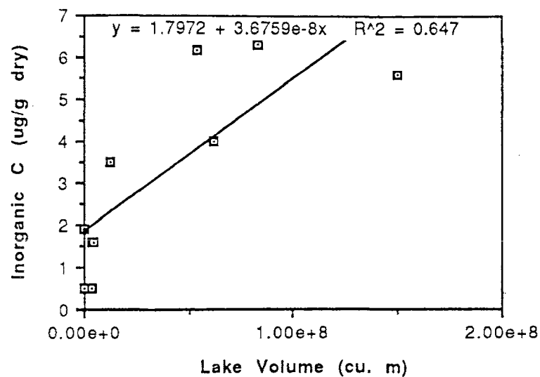
Figure 1: Inorganic C as a function of lake volume: northern Insular Belt.
