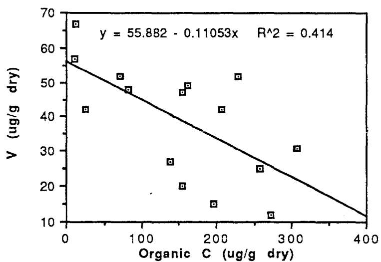
Figure 24: V as a function of organic C: southern Cascade Mountains.
