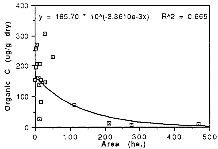
Figure 2: Organic C as a function of surface area: southern Cascade Mountains.
