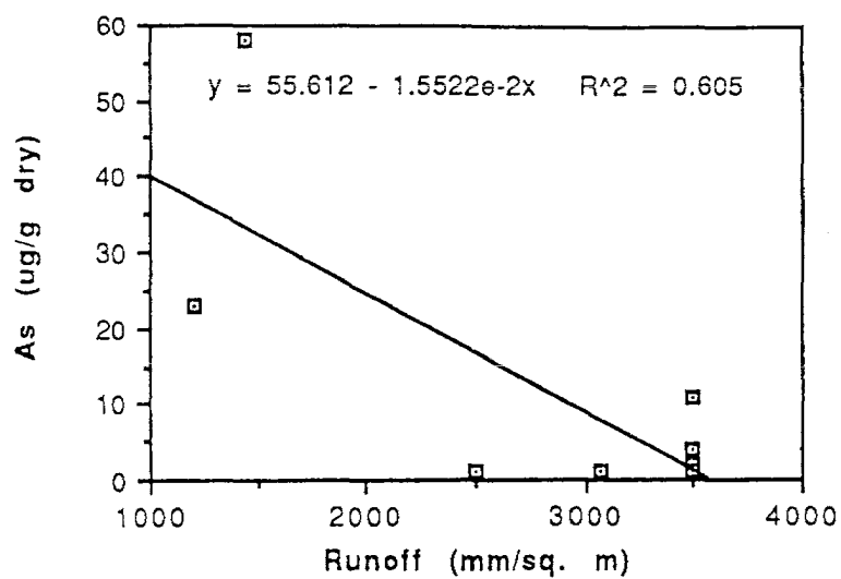
Figure 3: As as a function of runoff: northern Cascade Mountains.
