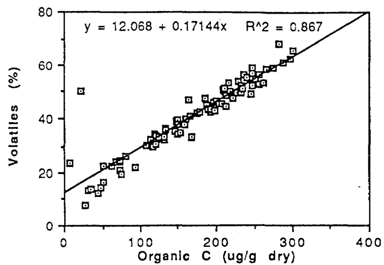
Figure 27: Volatiles as a function of organic C: southern Insular Belt.
