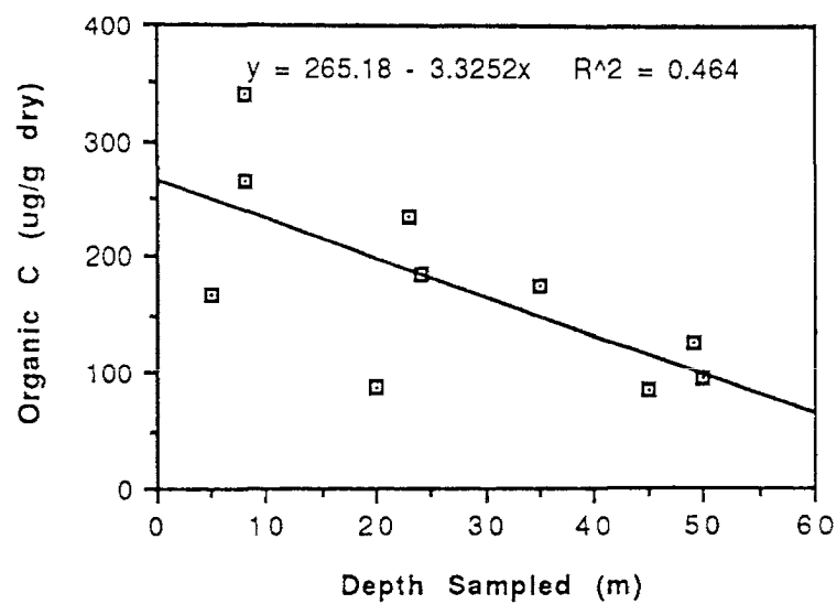
Figure 5: Organic C as a function of sample depth: northern Insular Belt.
