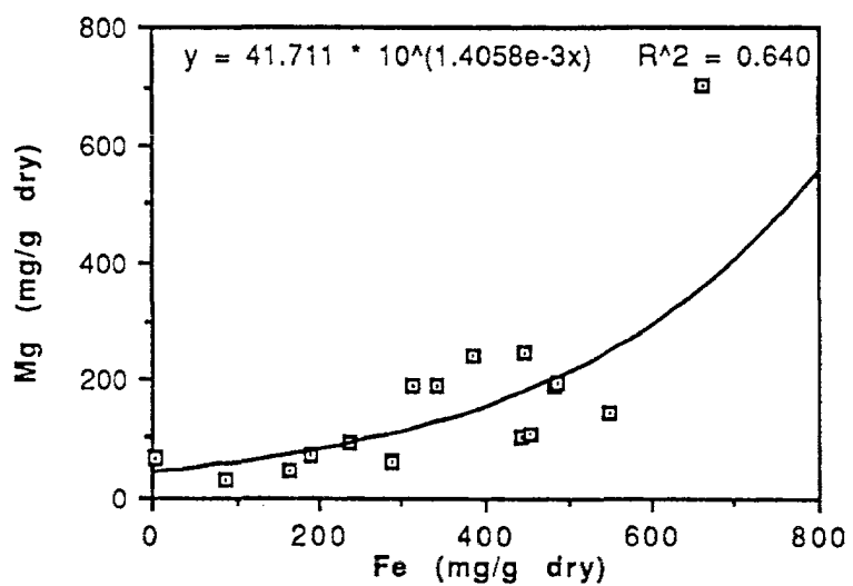
Figure 26: Mg as a function of Fe: northern Interior Plateau.
