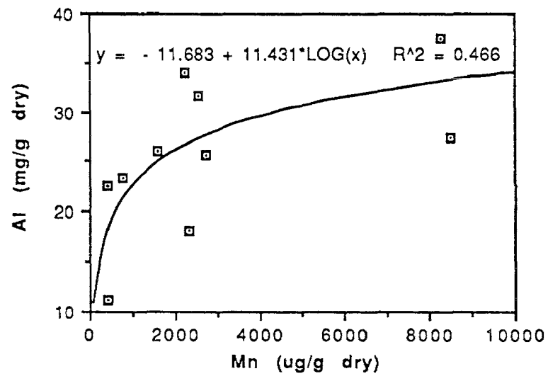
Figure 2: Al as a function of Mn: northern Insular Belt.
